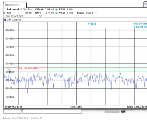
Band38-15MHz-QPSK-37825-1RB#0-Range1:0.009~0.15MHz
