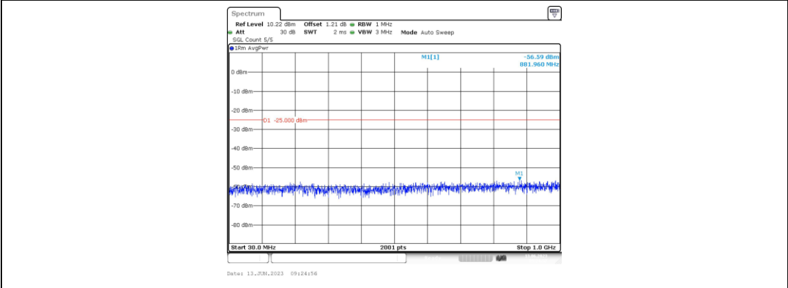
Band38-15MHz-16QAM-37825-1RB#0-Range3:30~1000MHz
