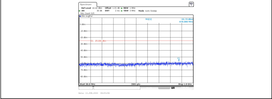
Band38-10MHz-16QAM-38000-1RB#0-Range3:30~1000MHz
