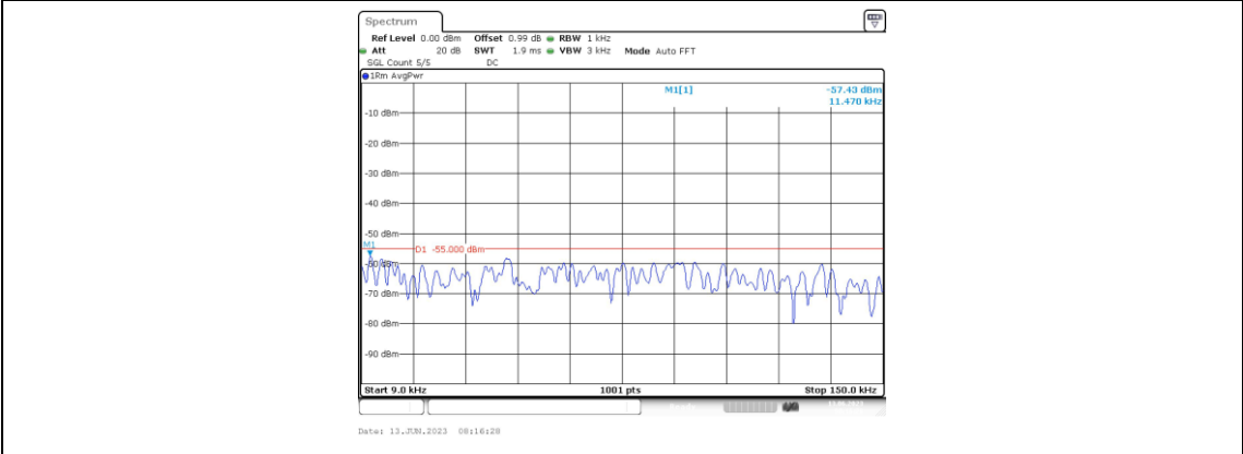
Band38-5MHz-16QAM-38225-1RB#0-Range1:0.009~0.15MHz
