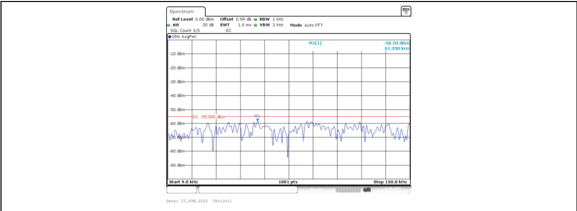
Band38-5MHz-QPSK-38000-1RB#0-Range1:0.009~0.15MHz
