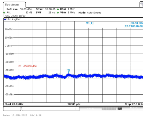
Band38-5MHz-QPSK-37775-1RB#0-Range5:20000~27000MHz
