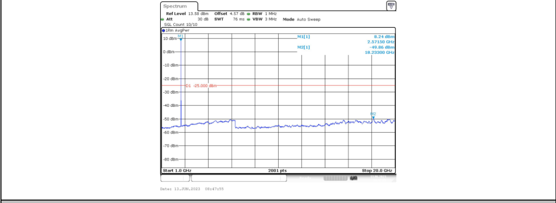
Band38-10MHz-QPSK-37800-1RB#0-Range4:1000~20000MHz
