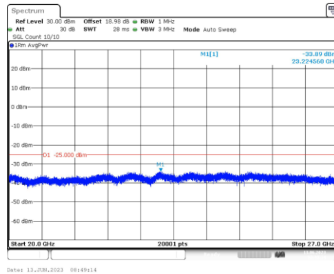
Band38-10MHz-16QAM-37800-1RB#0-Range5:20000~27000MHz
