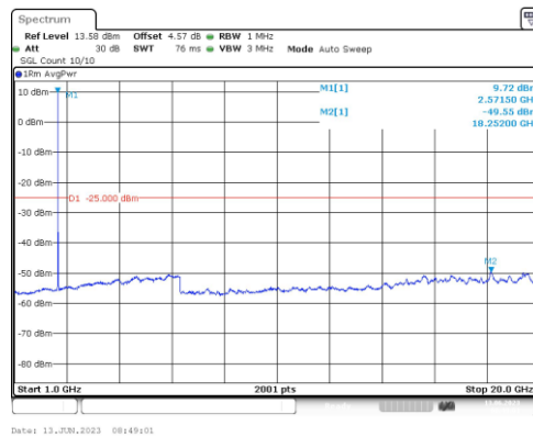
Band38-10MHz-16QAM-37800-1RB#0-Range4:1000~20000MHz
