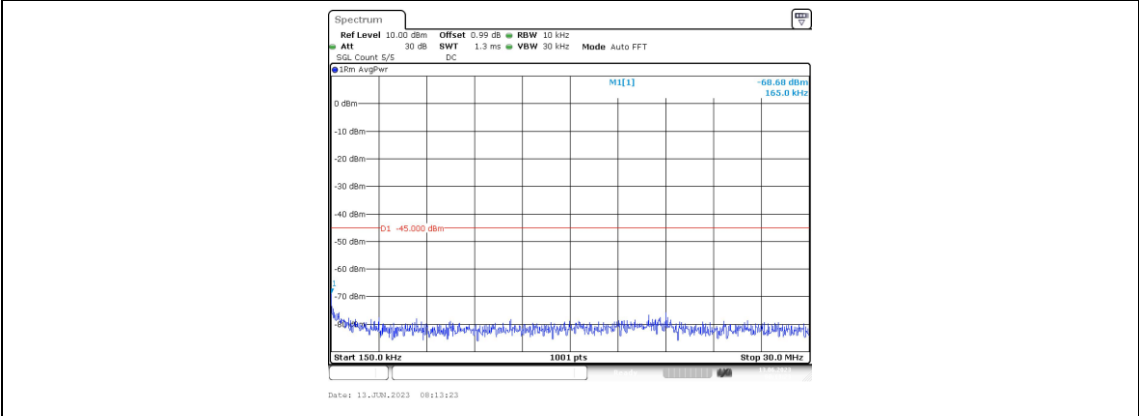
Band38-5MHz-QPSK-38000-1RB#0-Range2:0.15~30MHz
