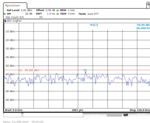
Band38-15MHz-QPSK-38175-1RB#0-Range1:0.009~0.15MHz
