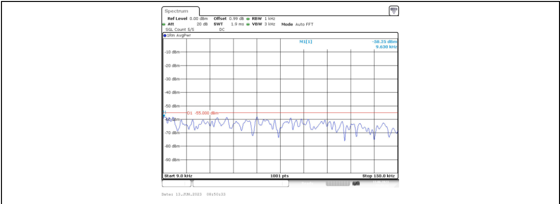
Band38-10MHz-16QAM-38000-1RB#0-Range1:0.009~0.15MHz
