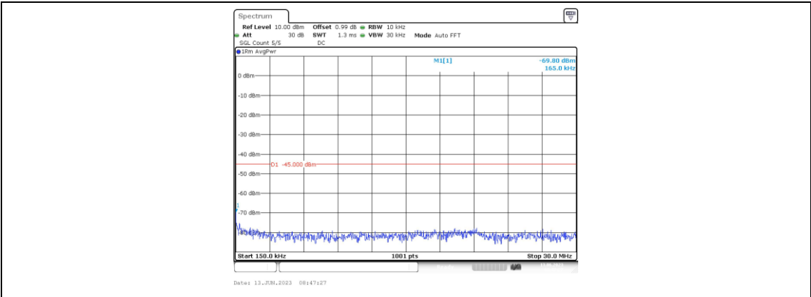
Band38-10MHz-QPSK-37800-1RB#0-Range2:0.15~30MHz
