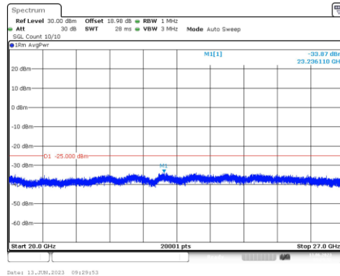
Band38-15MHz-16QAM-38175-1RB#0-Range5:20000~27000MHz
