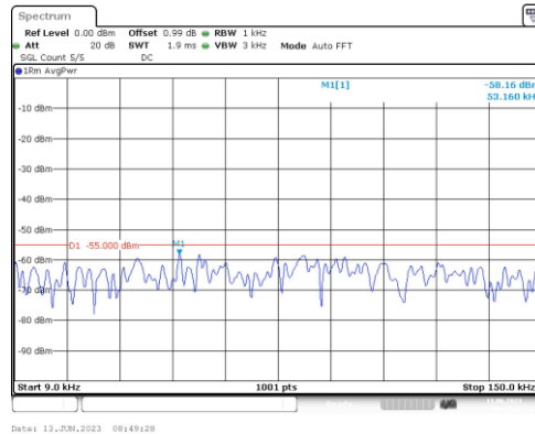
Band38-10MHz-QPSK-38000-1RB#0-Range1:0.009~0.15MHz
