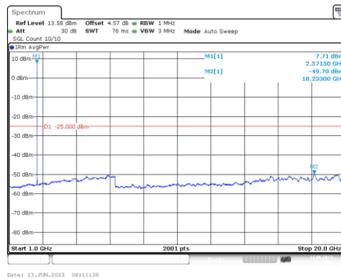
Band38-5MHz-QPSK-37775-1RB#0-Range4:1000~20000MHz
