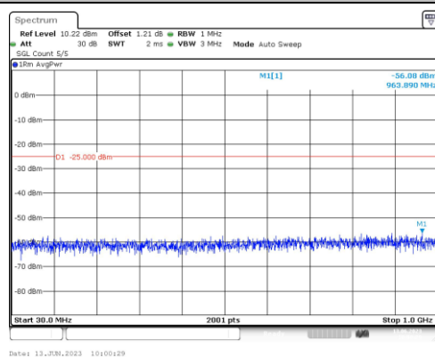
Band38-20MHz-QPSK-37850-1RB#0-Range3:30~1000MHz
