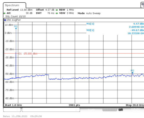
Band38-15MHz-16QAM-38175-1RB#0-Range4:1000~20000MHz
