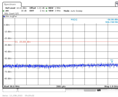
Band38-15MHz-16QAM-38175-1RB#0-Range3:30~1000MHz
