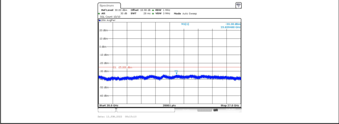
Band38-5MHz-16QAM-38000-1RB#0-Range5:20000~27000MHz
