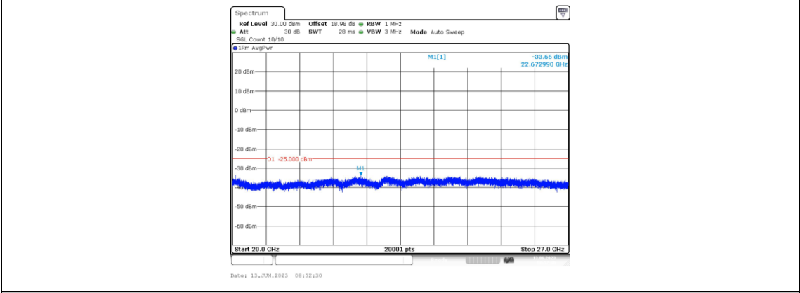
Band38-10MHz-QPSK-38200-1RB#0-Range5:20000~27000MHz
