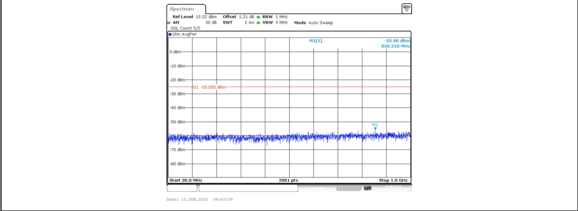
Band38-10MHz-QPSK-37800-1RB#0-Range3:30~1000MHz
