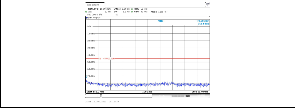
Band38-5MHz-16QAM-38225-1RB#0-Range2:0.15~30MHz
