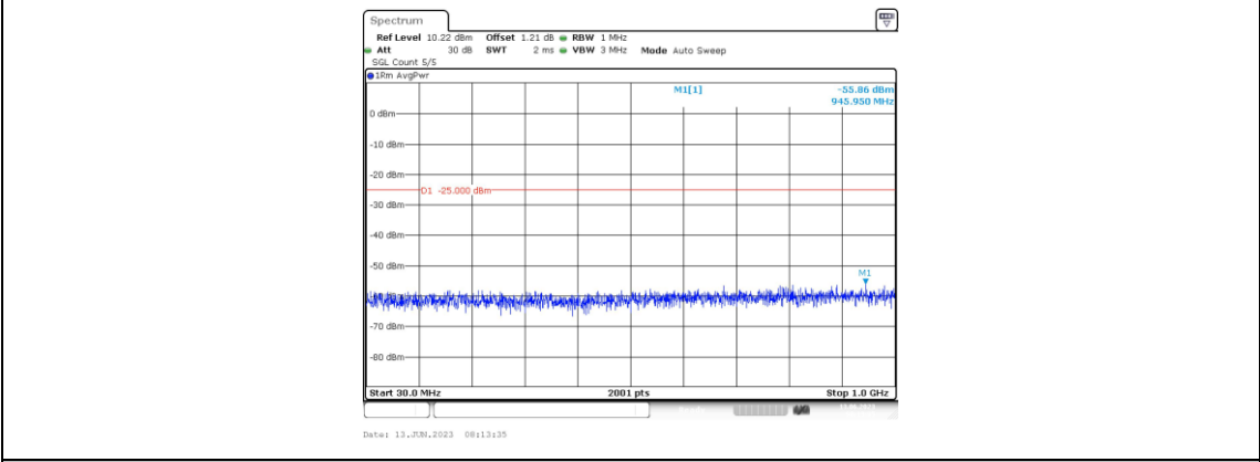
Band38-5MHz-QPSK-38000-1RB#0-Range3:30~1000MHz
