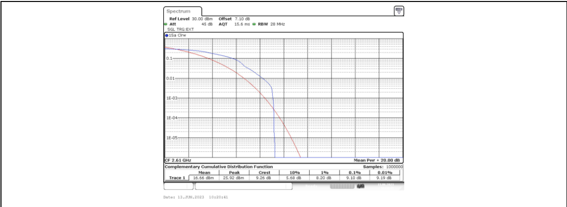
Band38-20MHz-16QAM-38150-1RB#0
