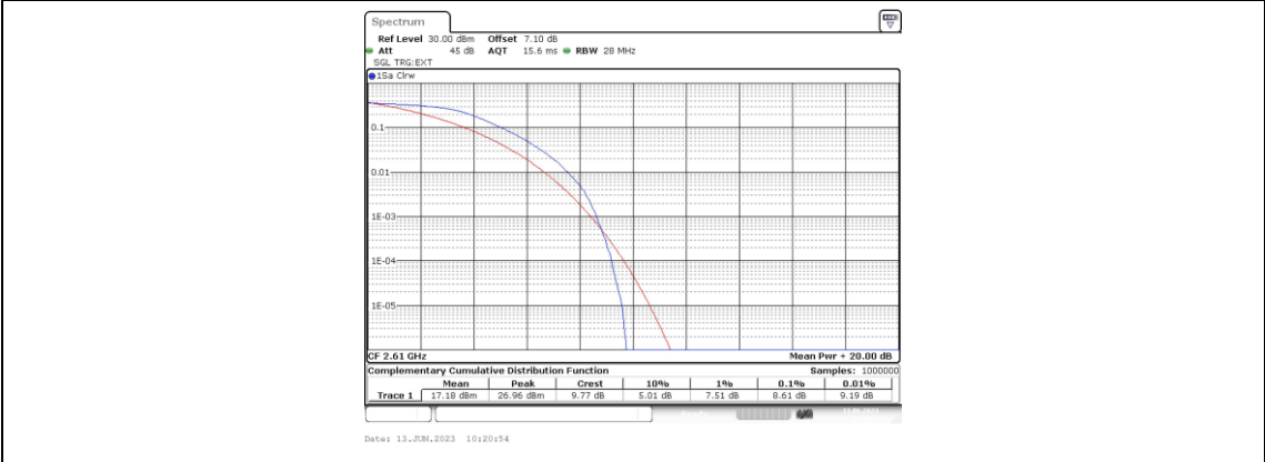
Band38-20MHz-QPSK-38150-100RB#0
