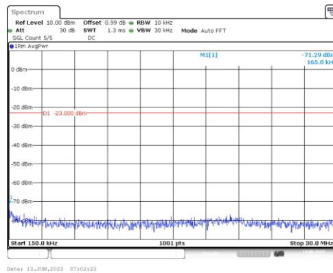
Band25-15MHz-16QAM-26115-1RB#0-Range2:0.15~30MHz
