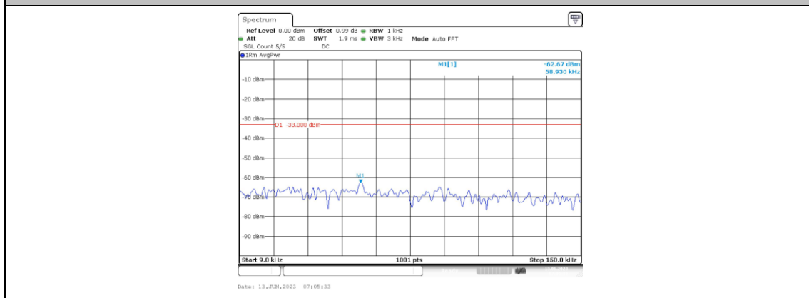
Band25-15MHz-16QAM-26615-1RB#0-Range1:0.009~0.15MHz
