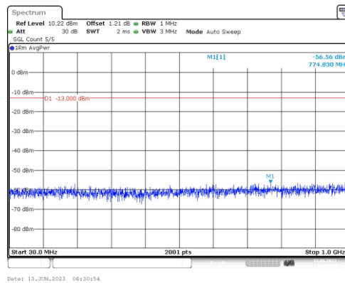
Band25-10MHz-16QAM-26365-1RB#0-Range3:30~1000MHz
