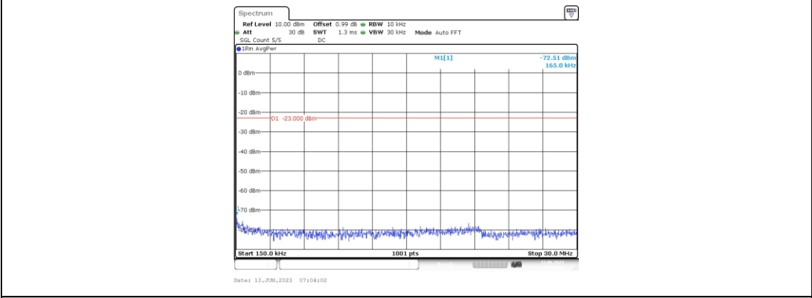
Band25-15MHz-16QAM-26365-1RB#0-Range2:0.15~30MHz
