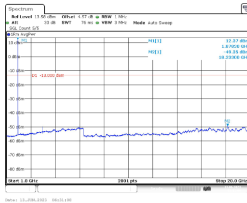
Band25-10MHz-16QAM-26365-1RB#0-Range4:1000~20000MHz
