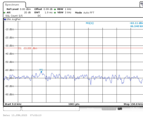
Band25-15MHz-16QAM-26115-1RB#0-Range1:0.009~0.15MHz
