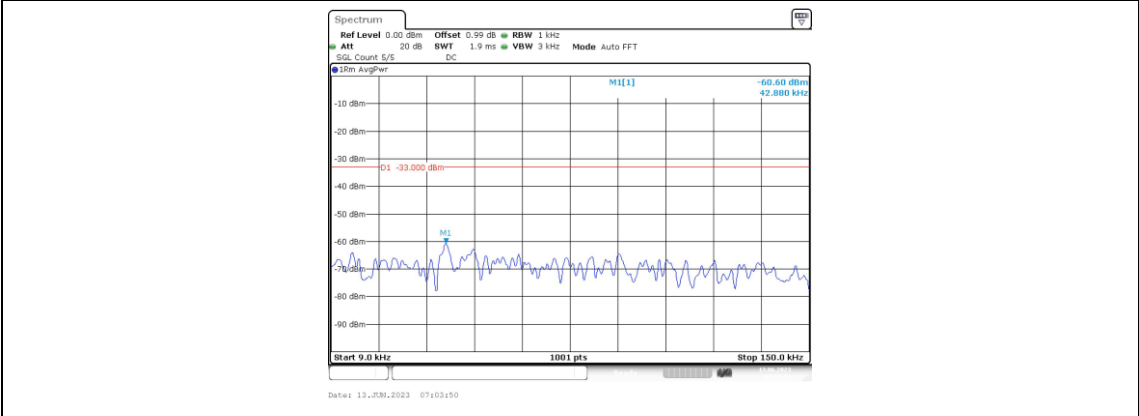
Band25-15MHz-16QAM-26365-1RB#0-Range1:0.009~0.15MHz
