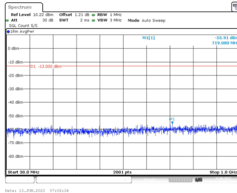
Band25-15MHz-16QAM-26115-1RB#0-Range3:30~1000MHz
