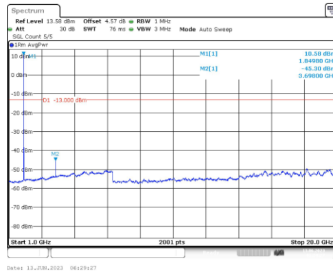
Band25-10MHz-16QAM-26090-1RB#0-Range4:1000~20000MHz
