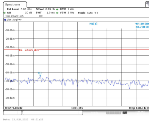
Band25-10MHz-QPSK-26640-1RB#0-Range1:0.009~0.15MHz
