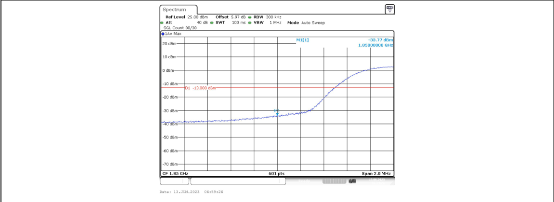
Band25-15MHz-16QAM-26115-75RB#0
