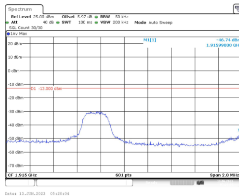
Band25-3MHz-16QAM-26675-1RB#0
