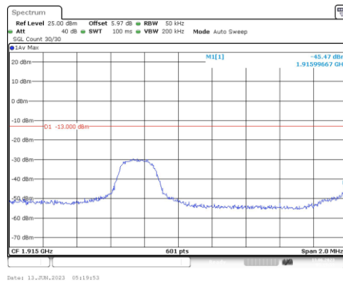
Band25-3MHz-QPSK-26675-1RB#0
