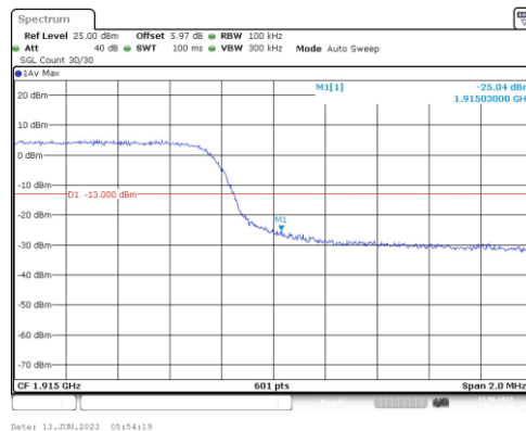
Band25-5MHz-16QAM-26665-1RB#24
