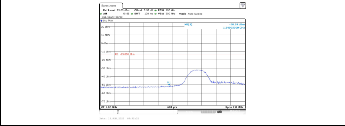
Band25-5MHz-QPSK-26065-1RB#24
