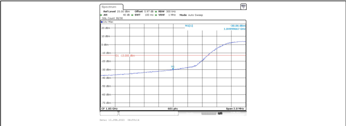
Band25-15MHz-QPSK-26115-75RB#0
