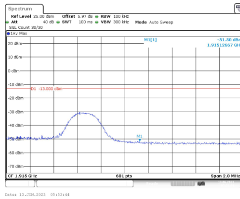
Band25-5MHz-16QAM-26665-1RB#0
