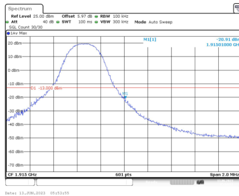
Band25-5MHz-QPSK-26665-1RB#24
