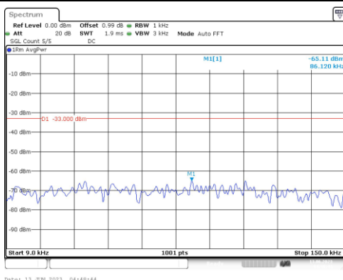
Band25-1.4MHz-QPSK-26047-1RB#0-Range1:0.009~0.15MHz
