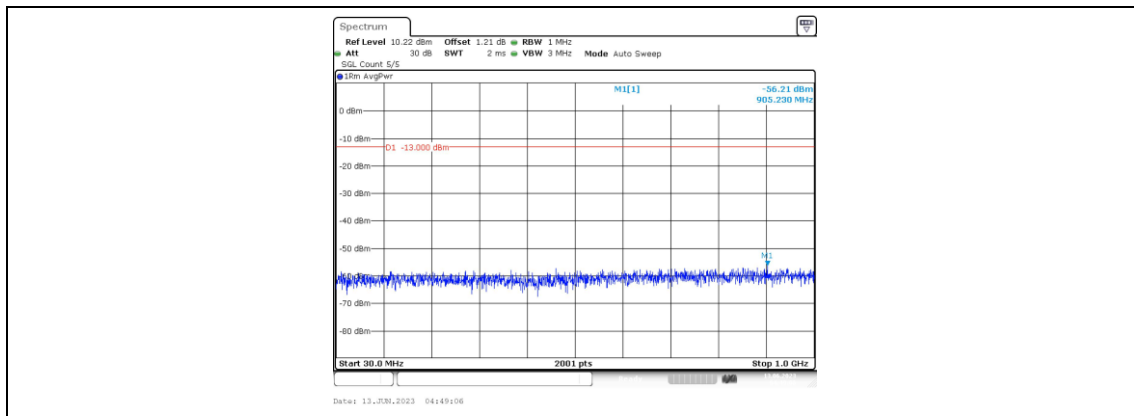
Band25.14MHz-QPSK-26047-1RB#0-Range3:30~1000MHz
