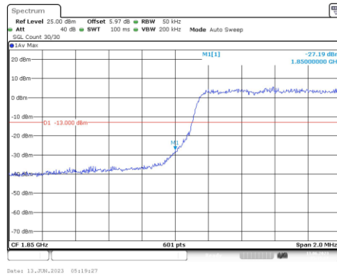
Band25-3MHz-16QAM-26055-15RB#0
