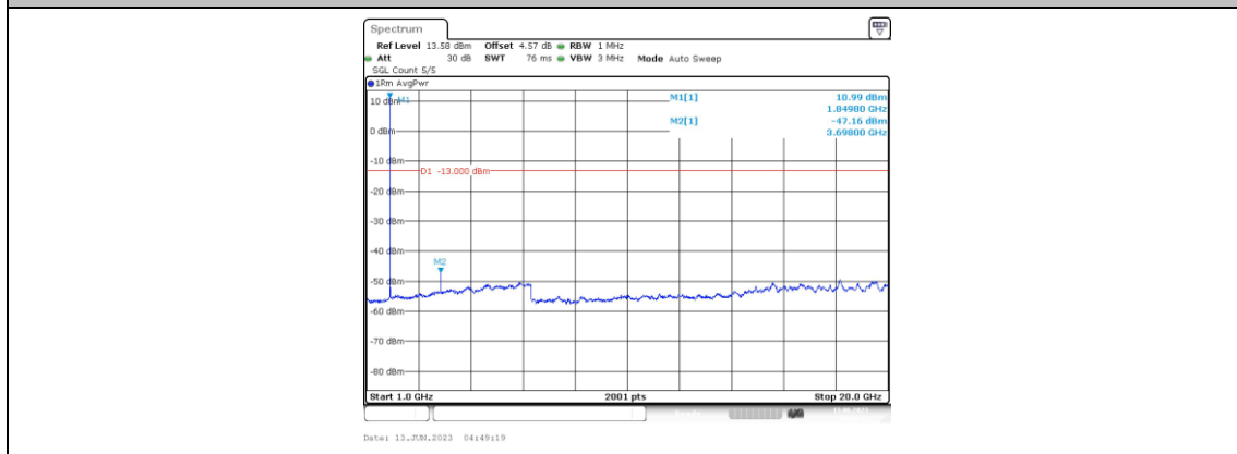
Band25.14MHz-QPSK-26047-1RB#0-Range4:1000~20000MHz
