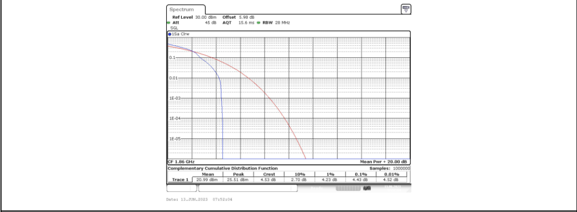
Band25-20MHz-16QAM-26140-1RB#0
