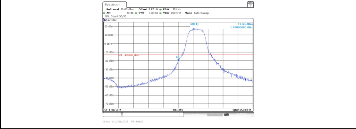
Band25-3MHz-QPSK-26055-1RB#0
