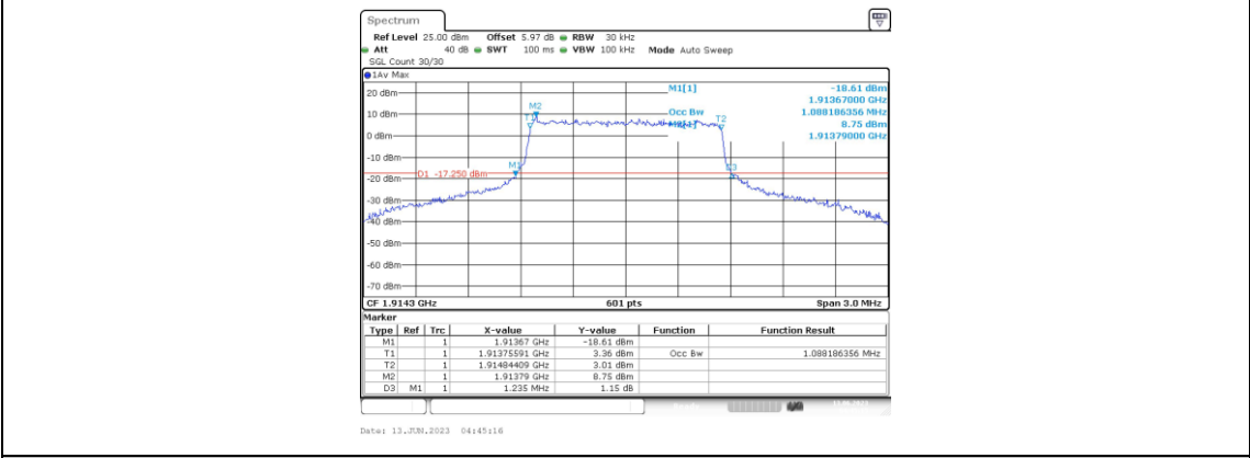
Band25-1.4MHz-16QAM-26683-6RB#0-1.088
