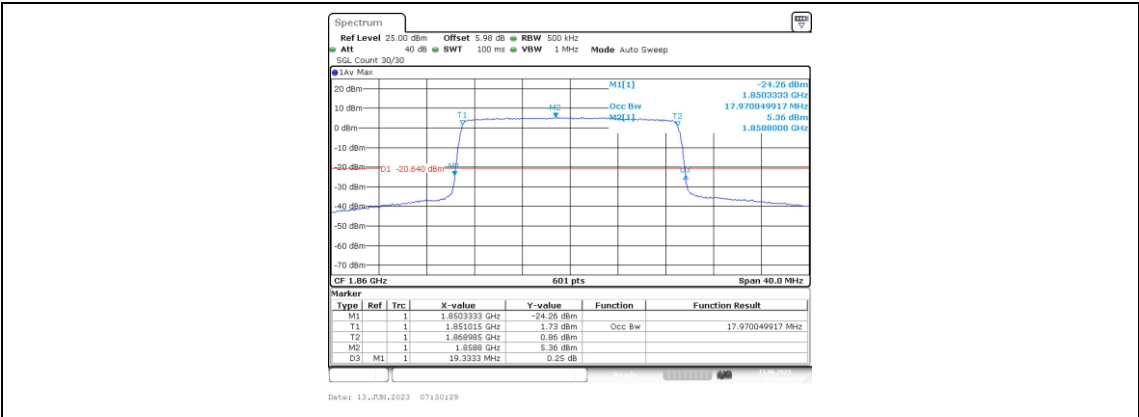
Band25-20MHz-16QAM-26140-100RB#0-17.97
