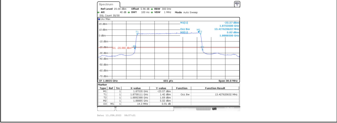
Band25-15MHz-QPSK-26365-75RB#0-13.428
