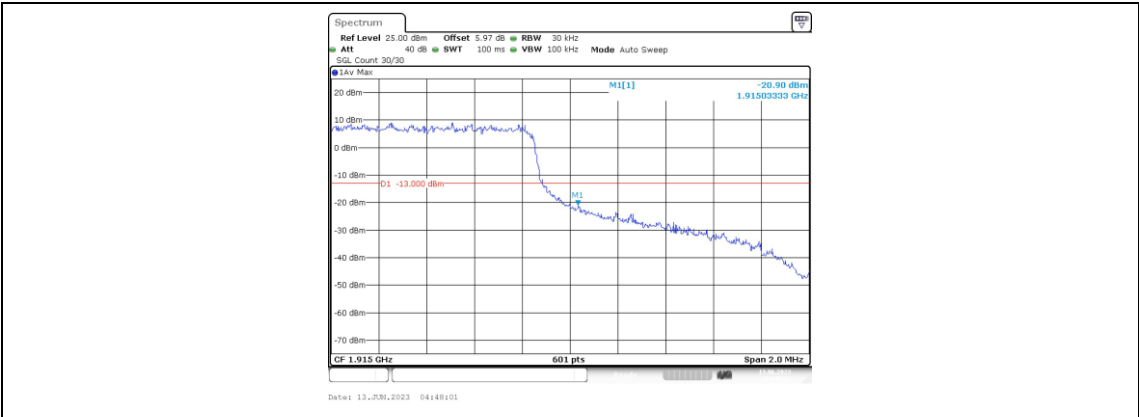
Band25-1.4MHz-QPSK-26683-6RB#0
