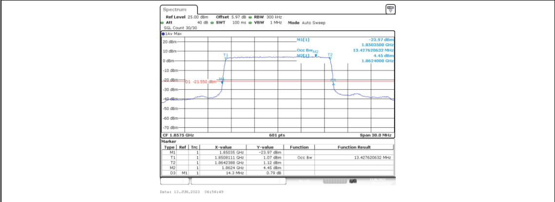
Band25-15MHz-16QAM-26115-75RB#0-13.428
