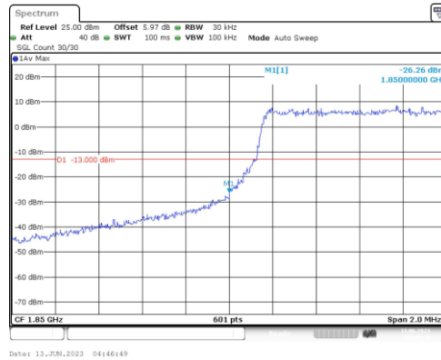
Band25-1.4MHz-16QAM-26047-6RB#0
