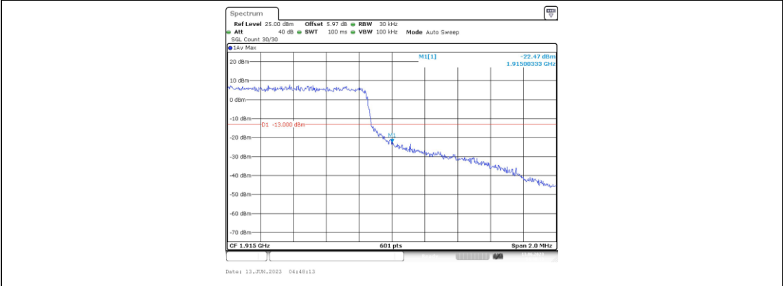
Band25-1.4MHz-16QAM-26683-6RB#0
