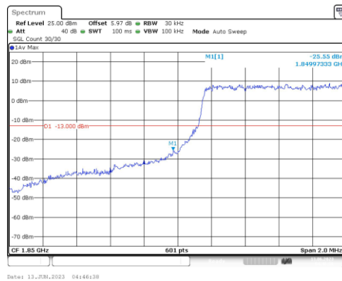
Band25-1.4MHz-QPSK-26047-6RB#0
