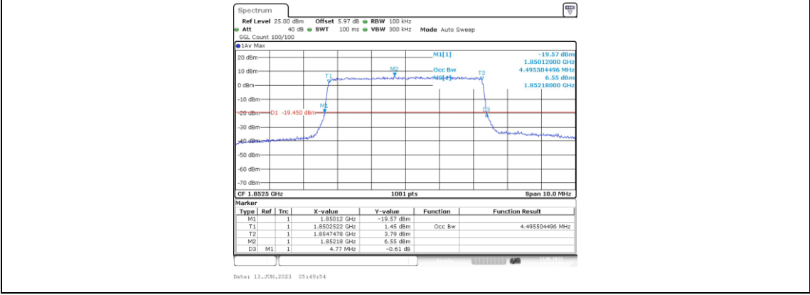
Band25-5MHz-QPSK-26065-25RB#0-4.496
