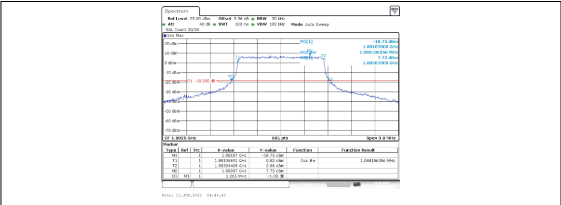
Band25-1.4MHz-16QAM-26365-6RB#0-1.088
