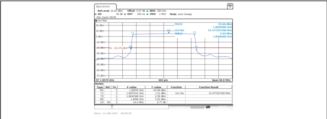
Band25-15MHz-QPSK-26115-75RB#0-13.478
