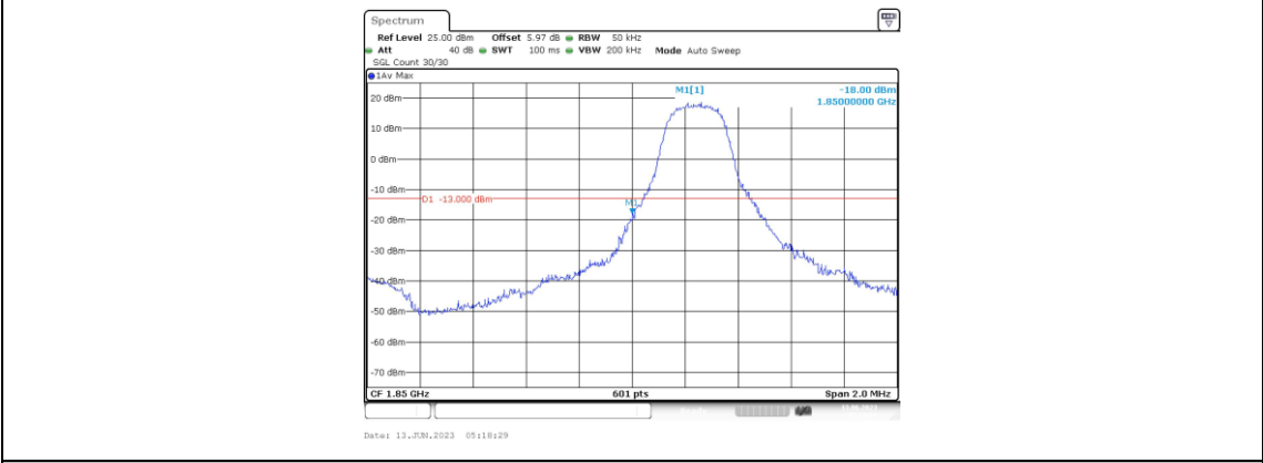
Band25-3MHz-QPSK-26055-1RB#0
