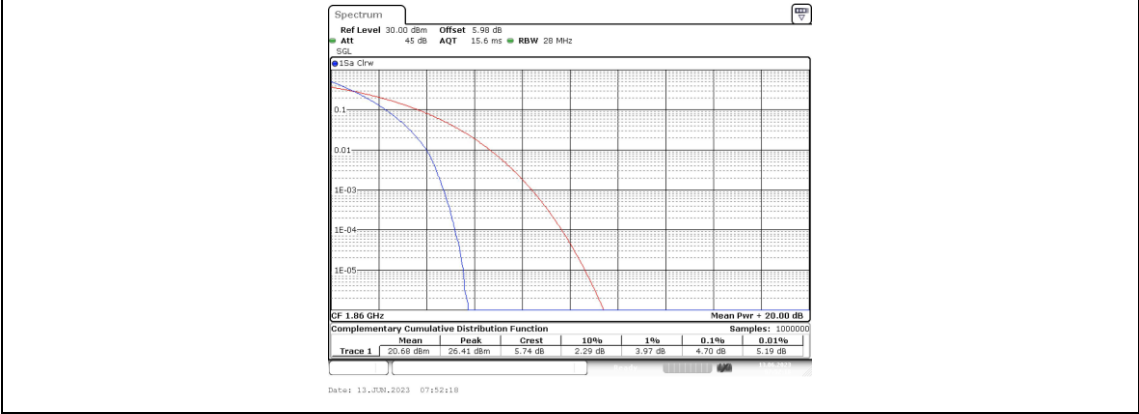
Band25-20MHz-16QAM-26140-1RB#0
