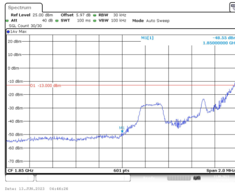
Band25-1.4MHz-16QAM-26047-1RB#5
