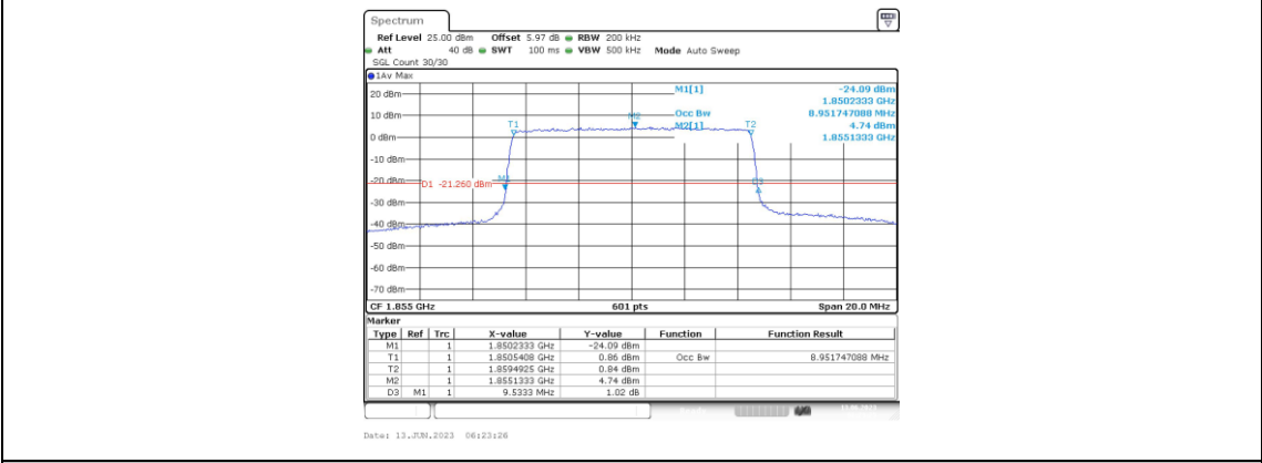
Band25-10MHz-16QAM-26090-50RB#0-8.952
