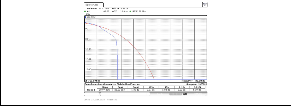
Band17-5MHz-16QAM-23790-1RB#0
