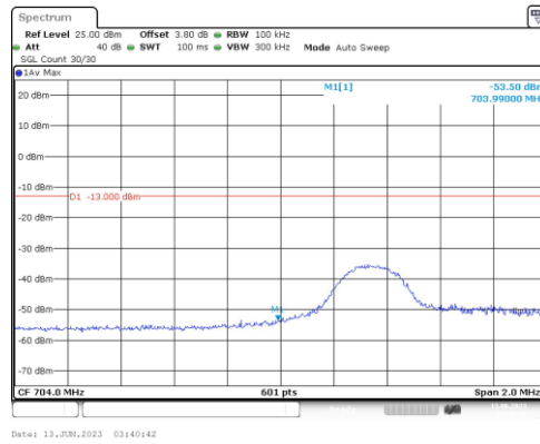
Band17-5MHz-16QAM-23755-1RB#24
