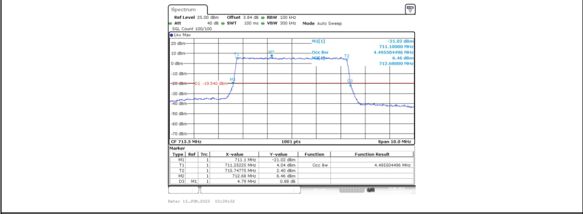
Band17-5MHz-16QAM-23825-25RB#0-4.496
