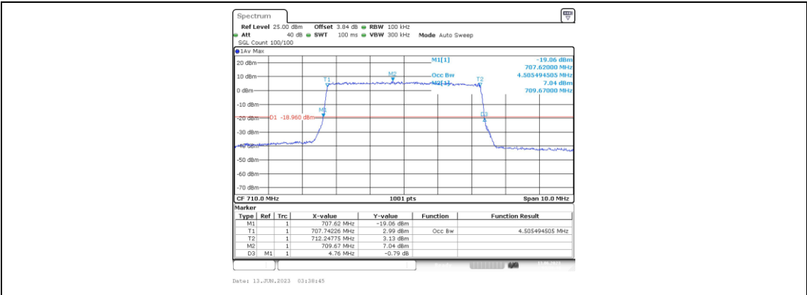
Band17-5MHz-16QAM-23790-25RB#0-4.505
