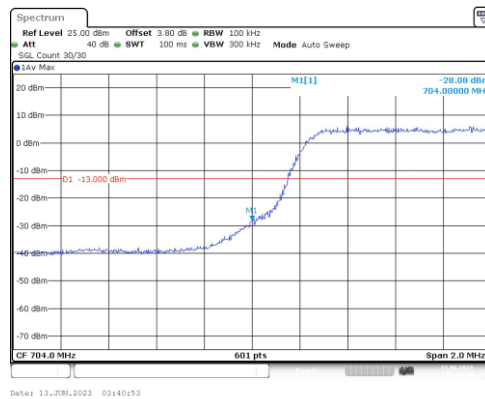
Band17-5MHz-QPSK-23755-25RB#0
