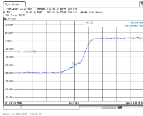
Band17-5MHz-16QAM-23755-25RB#0
