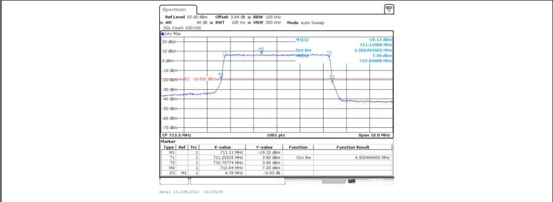
Band17-5MHz-QPSK-23825-25RB#0-4.505
