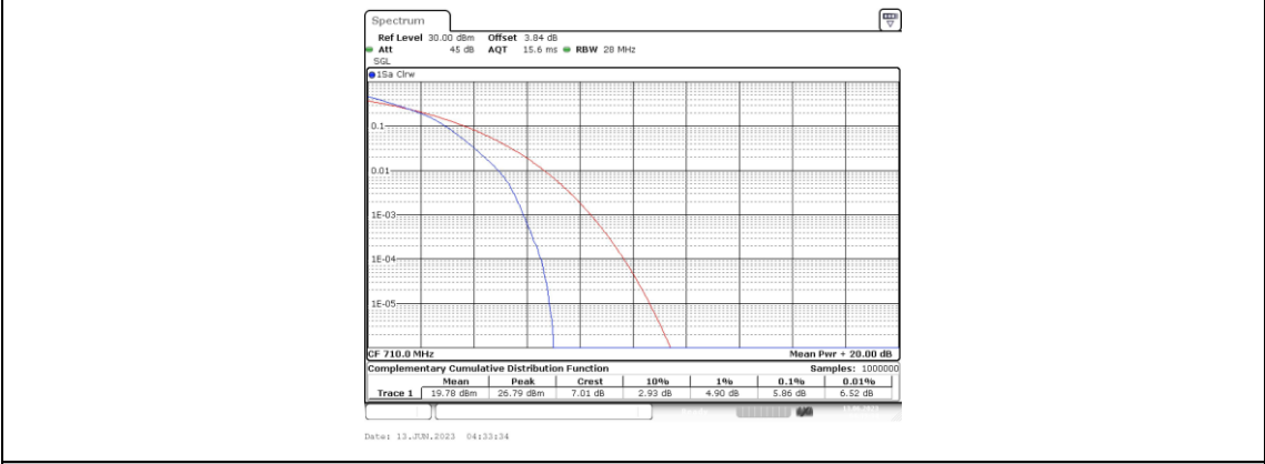
Band17-10MHz-16QAM-23790-50RB#0
