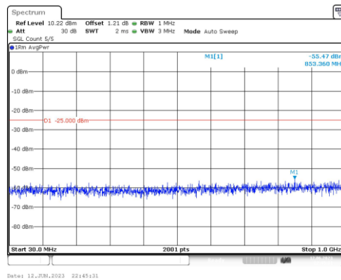
Band7-10MHz-QPSK-21400-1RB#0-Range3:30~1000MHz
