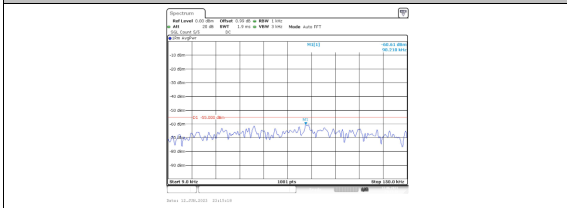
Band7-15MHz-QPSK-20825-1RB#0-Range1:0.009~0.15MHz
