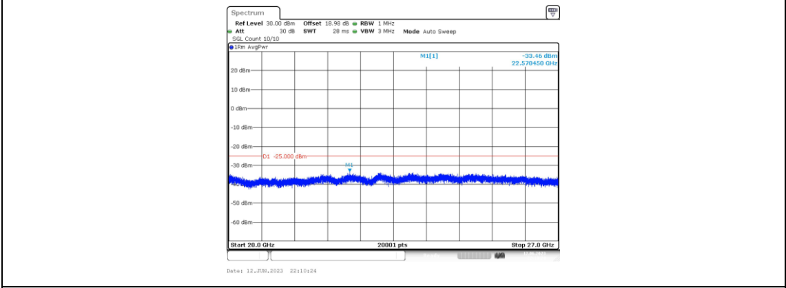
Band7-5MHz-16QAM-21100-1RB#0-Range5:20000~27000MHz
