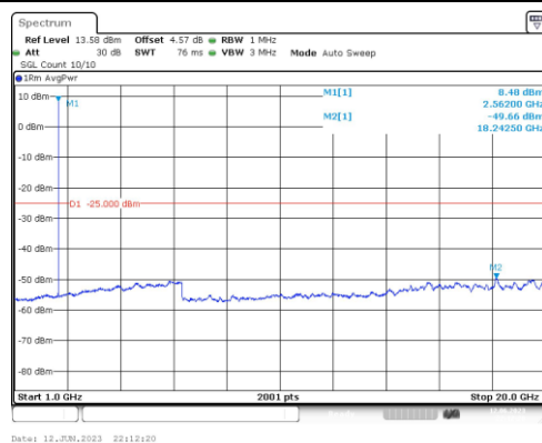
Band7-5MHz-16QAM-21425-1RB#0-Range4:1000~20000MHz
