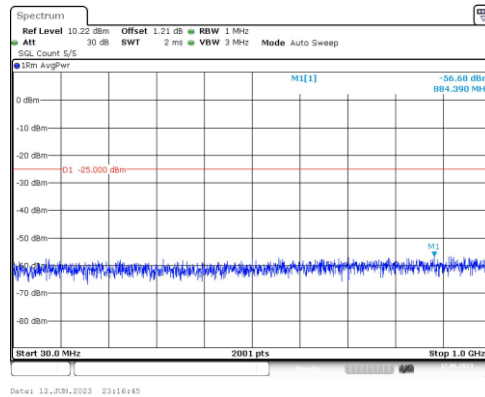
Band7-15MHz-16QAM-20825-1RB#0-Range3:30~1000MHz
