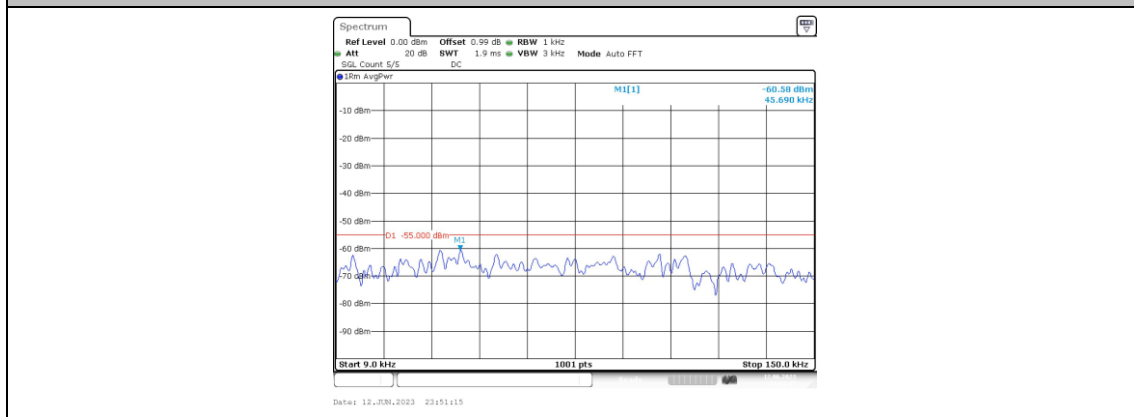
Band7-20MHz-16QAM-20850-1RB#0-Range1:0.009~0.15MHz
