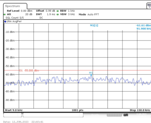
Band7-10MHz-QPSK-20800-1RB#0-Range1:0.009~0.15MHz
