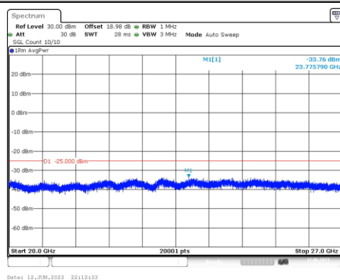
Band7-5MHz-16QAM-21425-1RB#0-Range5:20000~27000MHz
