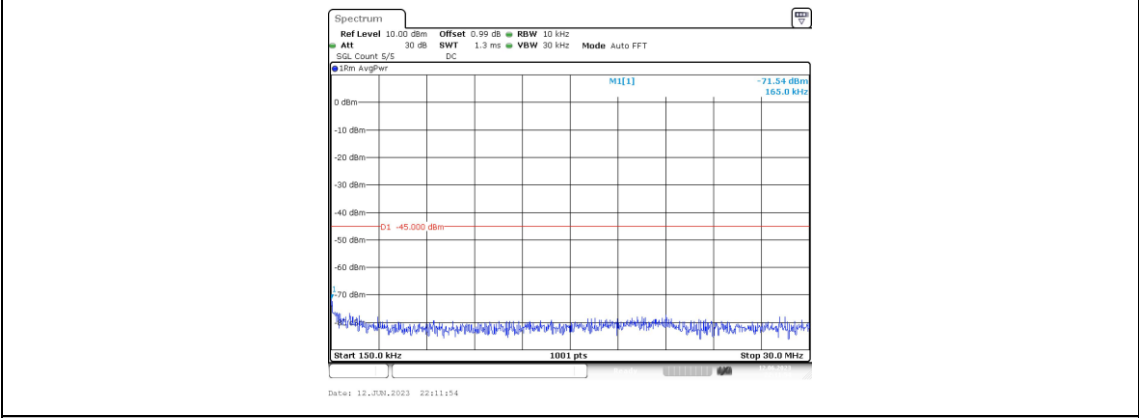
Band7-5MHz-16QAM-21425-1RB#0-Range2:0.15~30MHz
