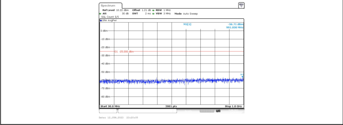
Band7-15MHz-QPSK-21375-1RB#0-Range3:30~1000MHz
