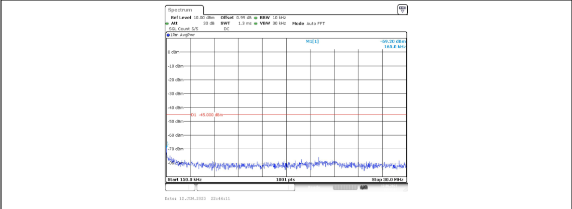
Band7-10MHz-16QAM-21100-1RB#0-Range2:0.15~30MHz
