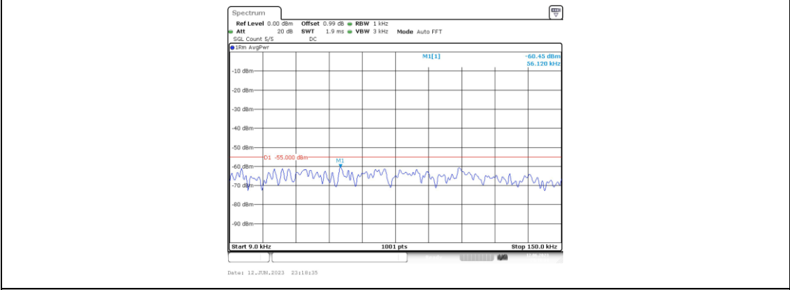
Band7-15MHz-16QAM-21100-1RB#0-Range1:0.009~0.15MHz
