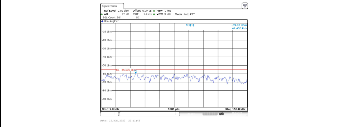
Band7-5MHz-16QAM-21425-1RB#0-Range1:0.009~0.15MHz
