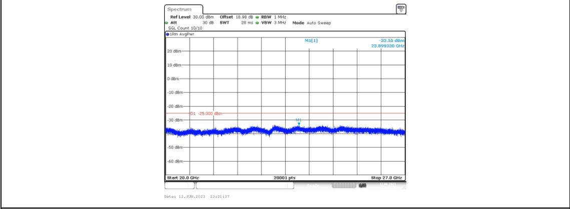
Band7-15MHz-16QAM-21375-1RB#0-Range5:20000~27000MHz
