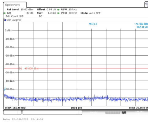
Band7-15MHz-16QAM-20825-1RB#0-Range2:0.15~30MHz
