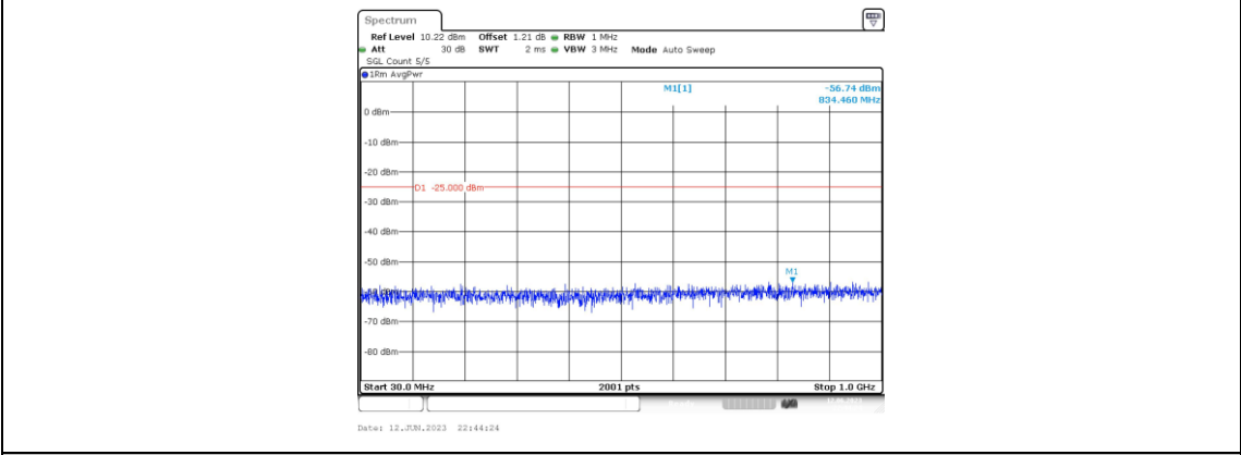
Band7-10MHz-16QAM-21100-1RB#0-Range3:30~1000MHz
