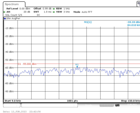
Band7-10MHz-QPSK-21100-1RB#0-Range1:0.009~0.15MHz
