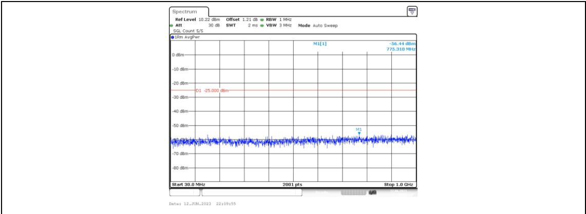
Band7-5MHz-16QAM-21100-1RB#0-Range3:30~1000MHz
