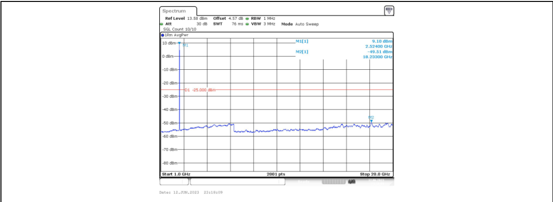
Band7-15MHz-QPSK-21100-1RB#0-Range4:1000~20000MHz
