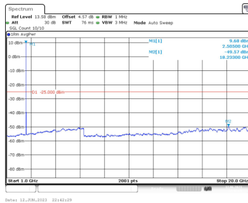
Band7-10MHz-16QAM-20800-1RB#0-Range4:1000~20000MHz
