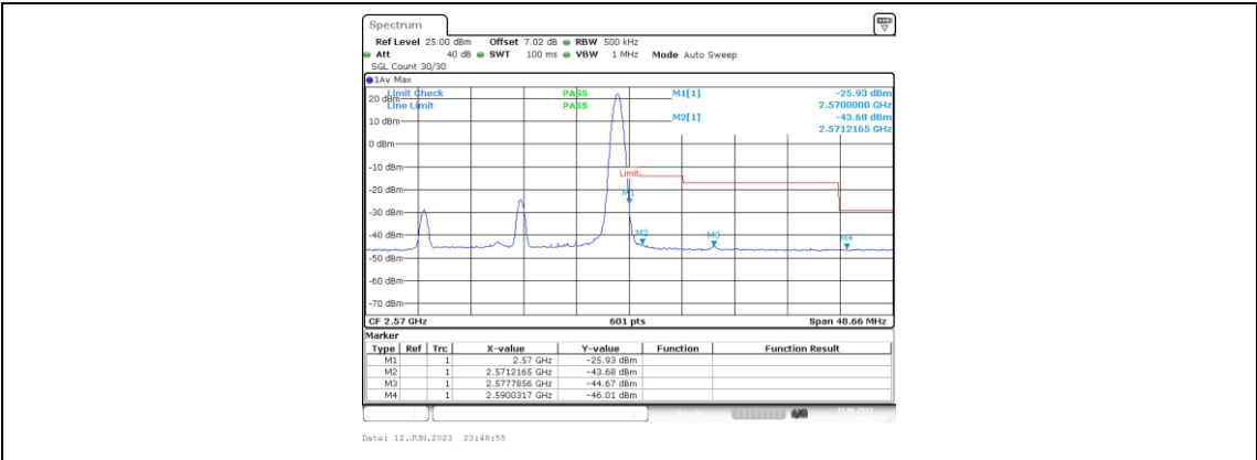
Band7-20MHz-QPSK-21350-1RB#99
