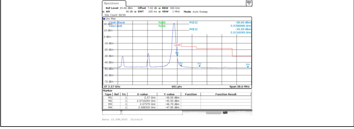
Band7-15MHz-QPSK-21375-1RB#74
