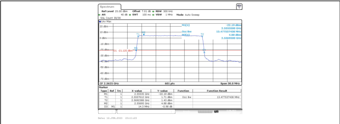
Band7-15MHz-16QAM-21375-75RB#0-13.478
