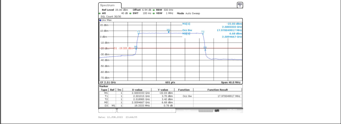
Band7-20MHz-QPSK-20850-100RB#0-17.97
