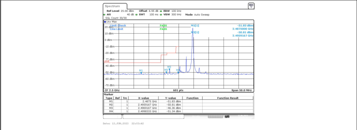
Band7-5MHz-16QAM-20775-1RB#24
