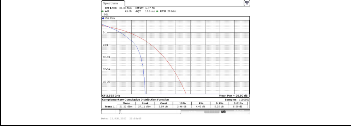
Band7-5MHz-16QAM-21100-1RB#0
