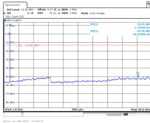
Band4-15MHz-QPSK-20325-1RB#0-Range4:1000~20000MHz
