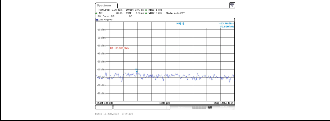
Band4-5MHz-16QAM-20375-1RB#0-Range1:0.009~0.15MHz
