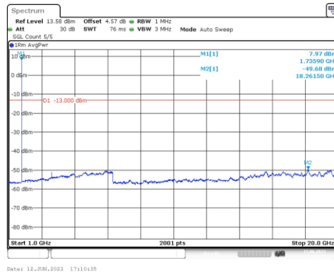
Band4-3MHz-16QAM-20175-1RB#0-Range4:1000~20000MHz
