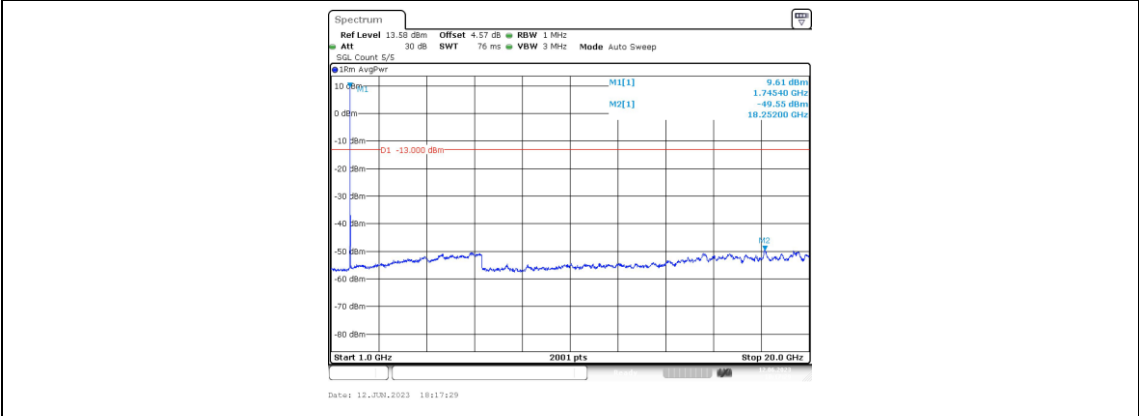
Band4-10MHz-16QAM-20350-1RB#0-Range4:1000~20000MHz
