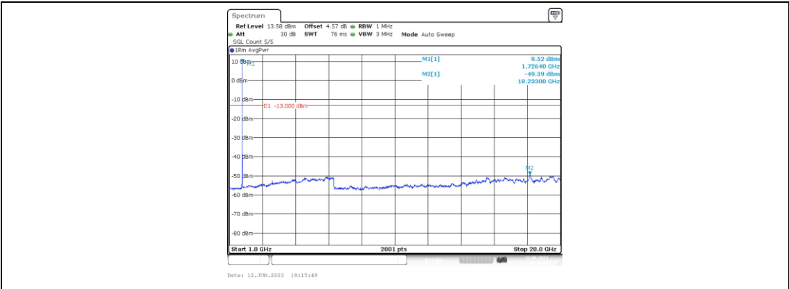
Band4-10MHz-16QAM-20175-1RB#0-Range4:1000~20000MHz
