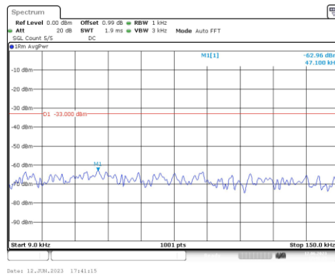
Band4-5MHz-16QAM-19975-1RB#0-Range1:0.009~0.15MHz
