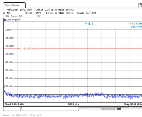
Band4-5MHz-16QAM-19975-1RB#0-Range2:0.15~30MHz
