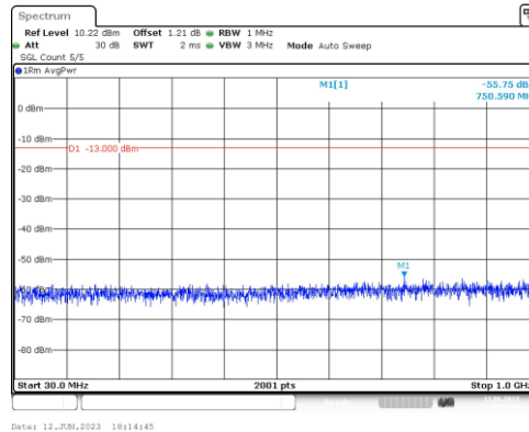
Band4-10MHz-QPSK-20175-1RB#0-Range3:30~1000MHz
