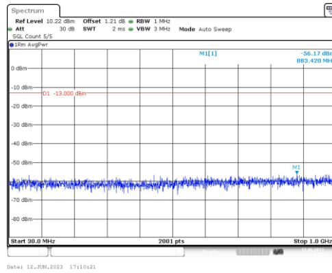
Band4-3MHz-16QAM-20175-1RB#0-Range3:30~1000MHz
