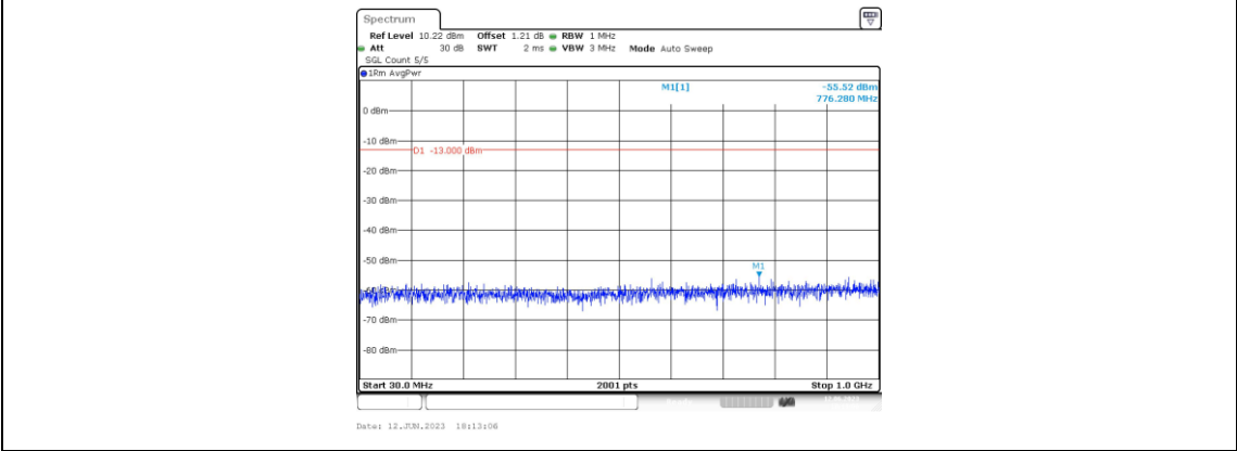
Band4-10MHz-QPSK-20000-1RB#0-Range3:30~1000MHz
