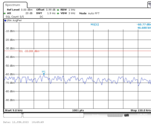
Band4-15MHz-16QAM-20325-1RB#0-Range1:0.009~0.15MHz
