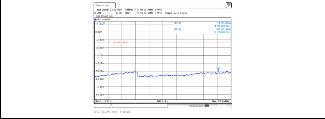
Band4-3MHz-16QAM-20385-1RB#0-Range4:1000~20000MHz
