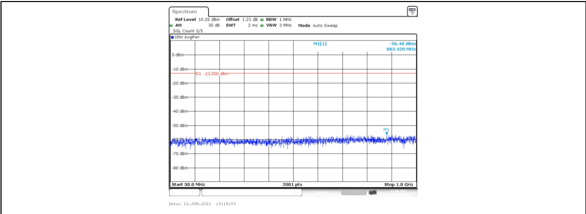
Band4-20MHz-QPSK-20050-1RB#0-Range3:30~1000MHz
