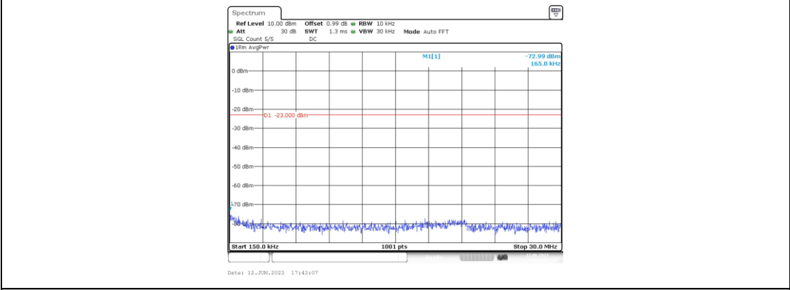
Band4-5MHz-16QAM-20175-1RB#0-Range2:0.15~30MHz
