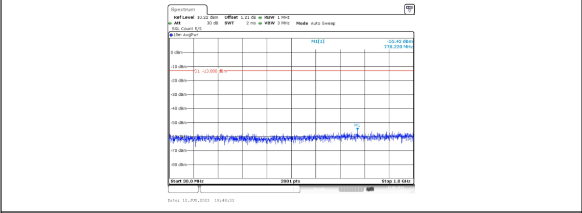
Band4-15MHz-16QAM-20175-1RB#0-Range3:30~1000MHz
