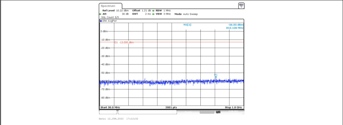
Band4-3MHz-16QAM-20385-1RB#0-Range3:30~1000MHz
