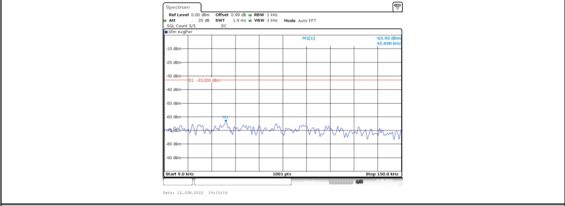
Band4-20MHz-16QAM-20050-1RB#0-Range1:0.009~0.15MHz
