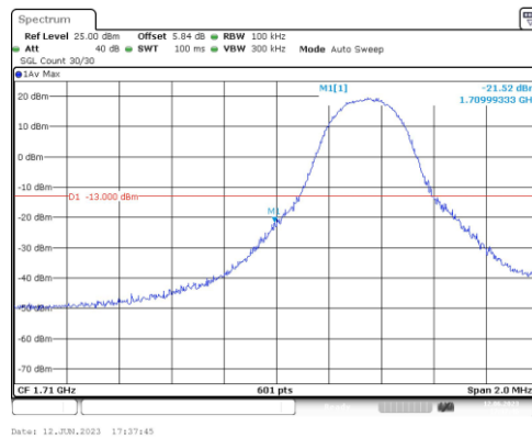
Band4-5MHz-16QAM-19975-1RB#0
