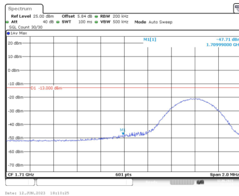
Band4-10MHz-16QAM-20000-1RB#49
