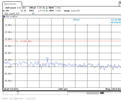
Band4-3MHz-QPSK-19965-1RB#0-Range1:0.009~0.15MHz
