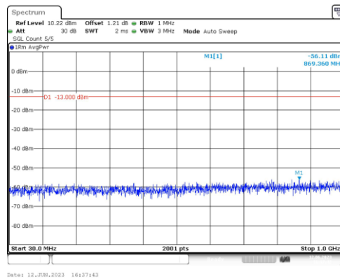
Band4-1.4MHz-QPSK-20175-1RB#0-Range3:30~1000MHz
