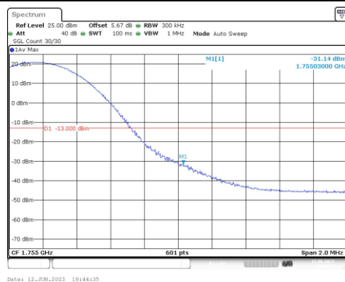
Band4-15MHz-QPSK-20325-1RB#74
