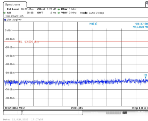
Band4-3MHz-QPSK-19965-1RB#0-Range3:30~1000MHz
