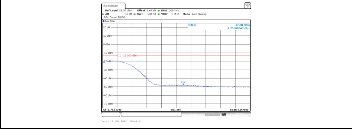
Band4-15MHz-QPSK-20325-1RB#0
