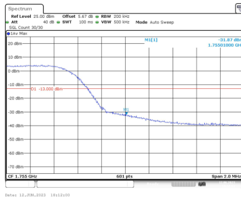
Band4-10MHz-QPSK-20350-50RB#0
