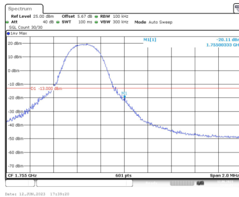
Band4-5MHz-QPSK-20375-1RB#24
