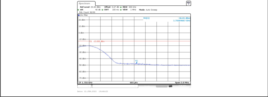
Band4-15MHz-QPSK-20325-1RB#0
