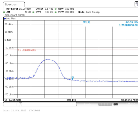
Band4-5MHz-16QAM-20375-1RB#0
