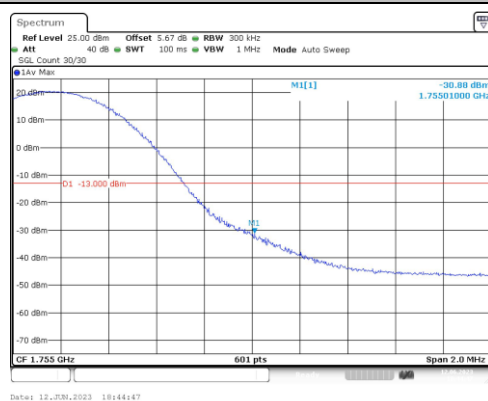
Band4-15MHz-16QAM-20325-1RB#74
