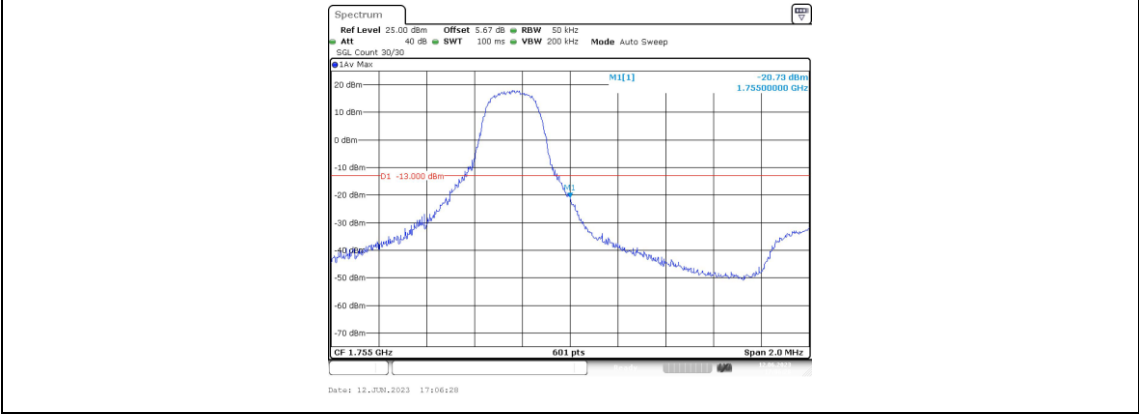
Band4-3MHz-16QAM-20385-1RB#0
