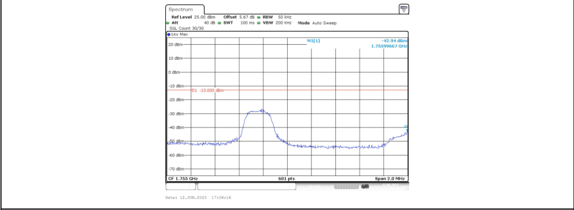
Band4-3MHz-16QAM-20385-1RB#0
