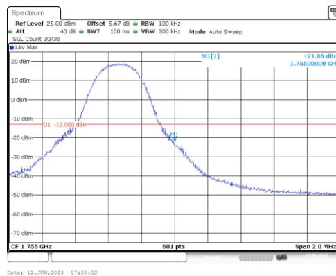
Band4-5MHz-16QAM-20375-1RB#24
