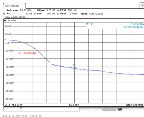
Band4-15MHz-QPSK-20325-75RB#0
