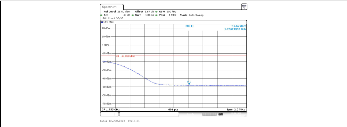
Band4-20MHz-QPSK-20300-1RB#0
