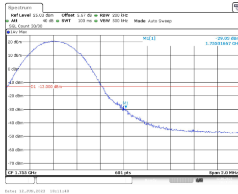
Band4-10MHz-16QAM-20350-1RB#49
