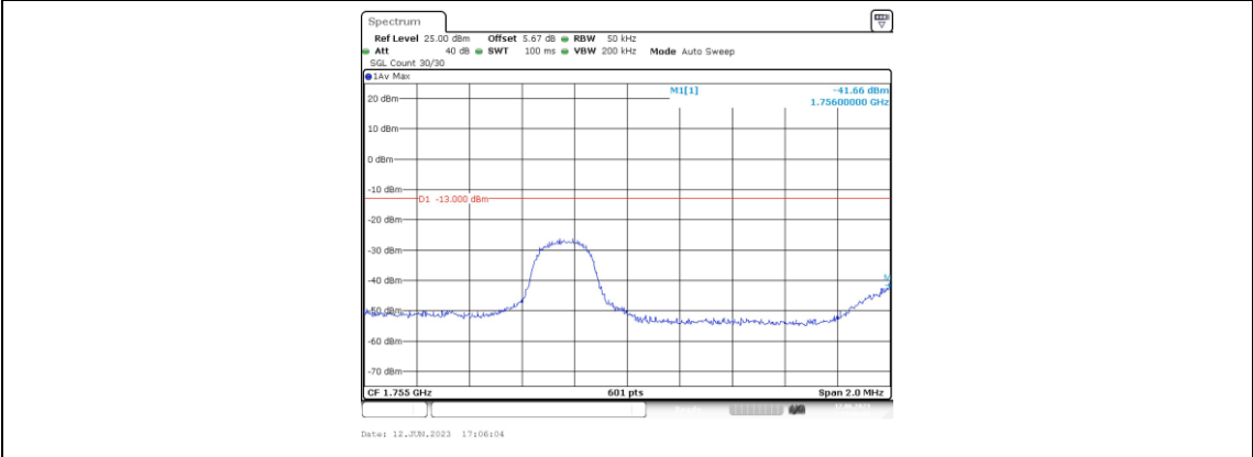
Band4-3MHz-QPSK-20385-1RB#0
