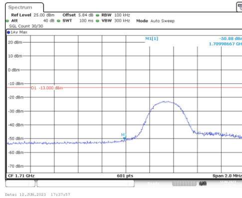
Band4-5MHz-QPSK-19975-1RB#24
