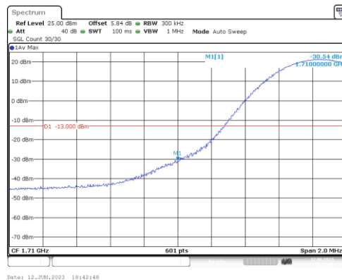
Band4-10MHz-16QAM-20350-50RB#0
