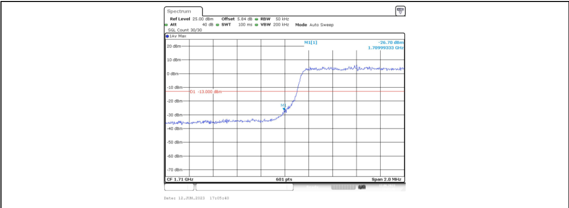
Band4-3MHz-16QAM-19965-15RB#0
