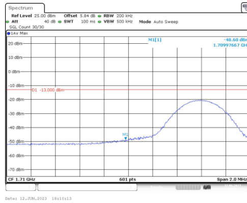
Band4-10MHz-QPSK-20000-1RB#49
