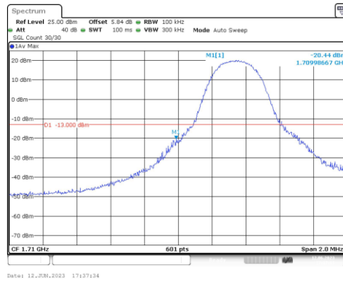
Band4-5MHz-QPSK-19975-1RB#0
