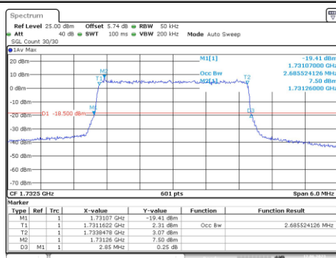
Band4-3MHz-16QAM-19965-15RB#0-2.686
