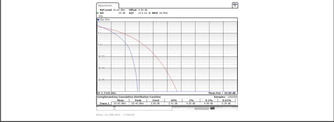
Band4-5MHz-QPSK-19975-25RB#0
