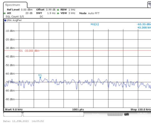
Band2-5MHz-16QAM-18900-1RB#0-Range1:0.009~0.15MHz
