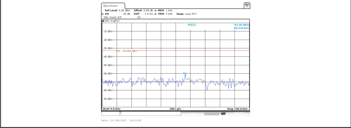
Band2-20MHz-16QAM-18700-1RB#0-Range1:0.009~0.15MHz
