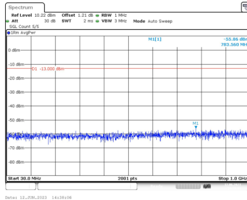
Band2-10MHz-QPSK-18900-1RB#0-Range3:30~1000MHz
