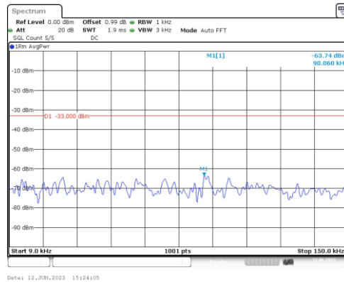
Band2-15MHz-16QAM-19125-1RB#0-Range1:0.009~0.15MHz
