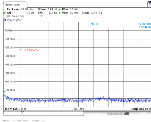
Band2-5MHz-16QAM-18900-1RB#0-Range2:0.15~30MHz
