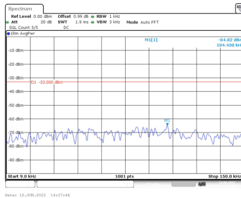
Band2-10MHz-QPSK-18900-1RB#0-Range1:0.009~0.15MHz
