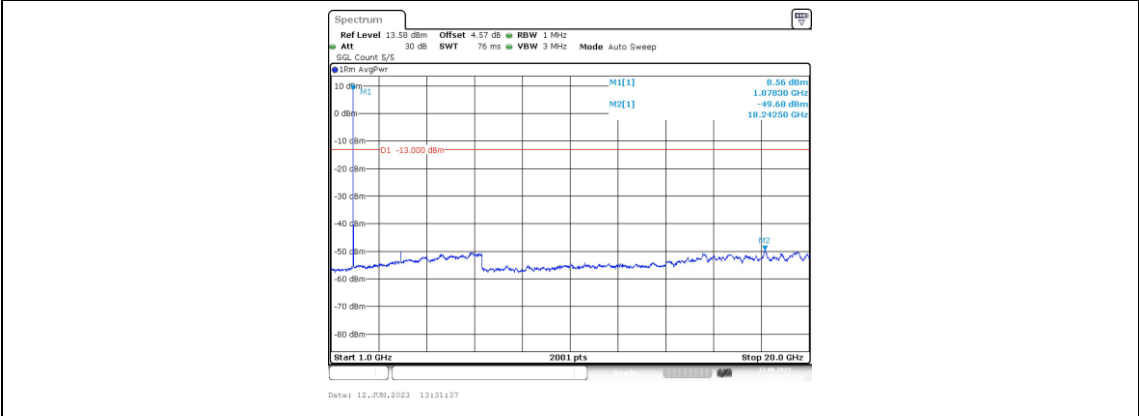
Band2-3MHz-16QAM-18900-1RB#0-Range4:1000~20000MHz
