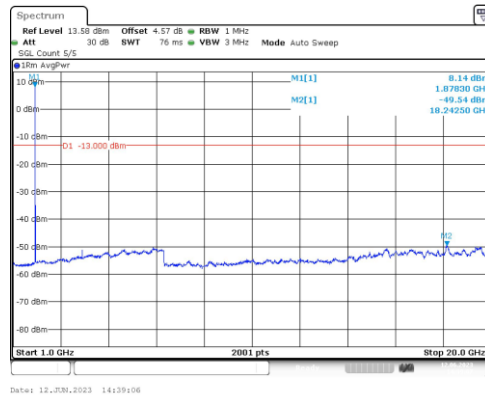
Band2-10MHz-16QAM-18900-1RB#0-Range4:1000~20000MHz
