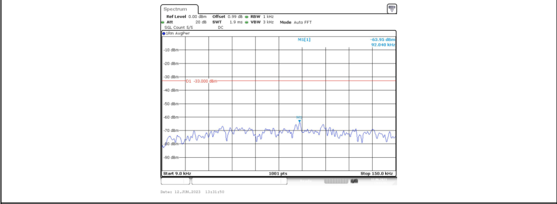
Band2-3MHz-QPSK-19185-1RB#0-Range1:0.009~0.15MHz
