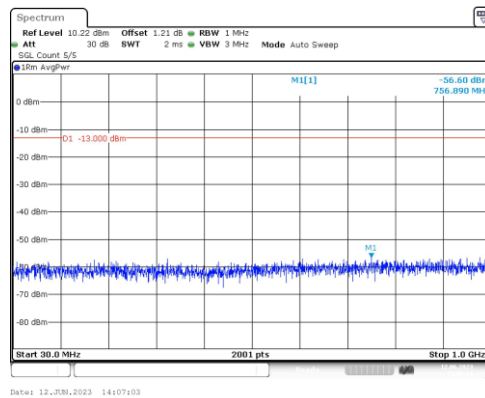
Band2-5MHz-QPSK-19175-1RB#0-Range3:30~1000MHz
