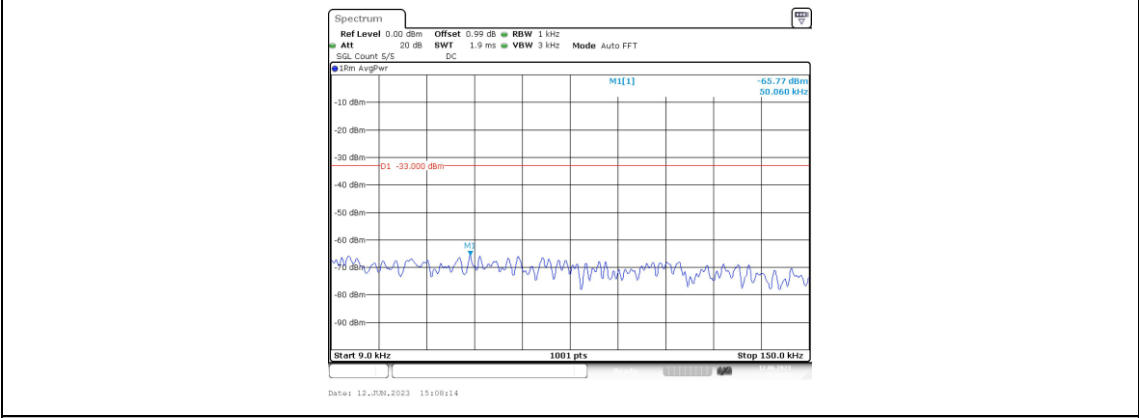
Band2-15MHz-QPSK-18675-1RB#0-Range1:0.009~0.15MHz
