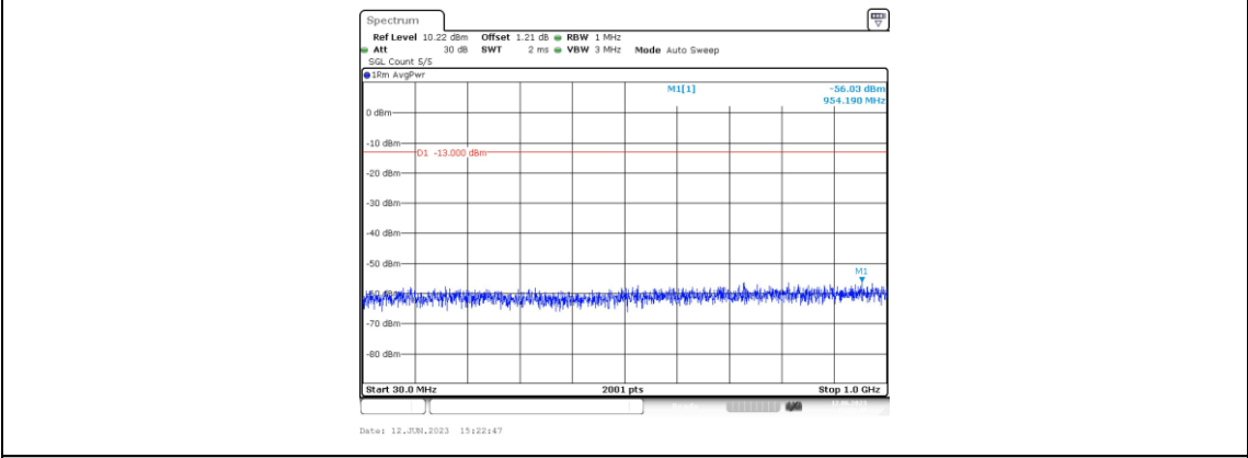
Band2-15MHz-16QAM-18900-1RB#0-Range3:30~1000MHz
