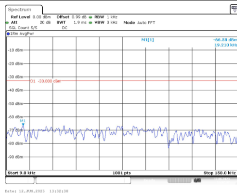
Band2-3MHz-16QAM-19185-1RB#0-Range1:0.009~0.15MHz
