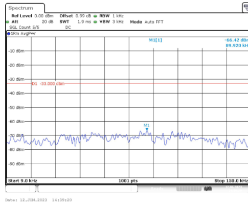
Band2-10MHz-QPSK-19150-1RB#0-Range1:0.009~0.15MHz
