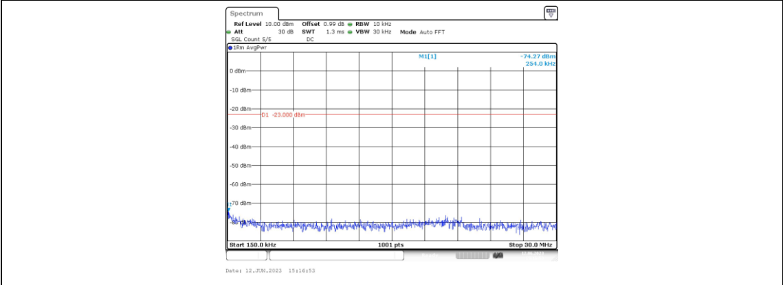
Band2-15MHz-16QAM-18900-1RB#0-Range2:0.15~30MHz
