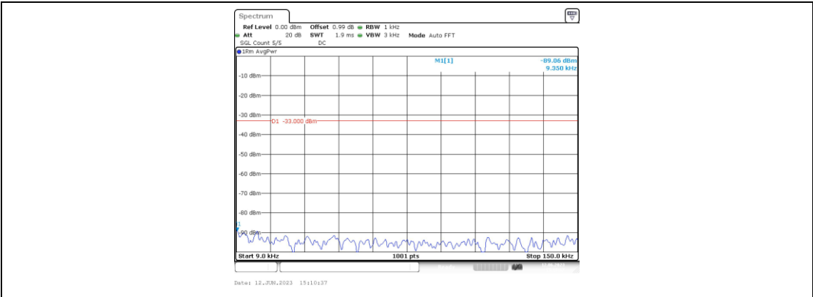
Band2-15MHz-16QAM-18900-1RB#0-Range1:0.009~0.15MHz
