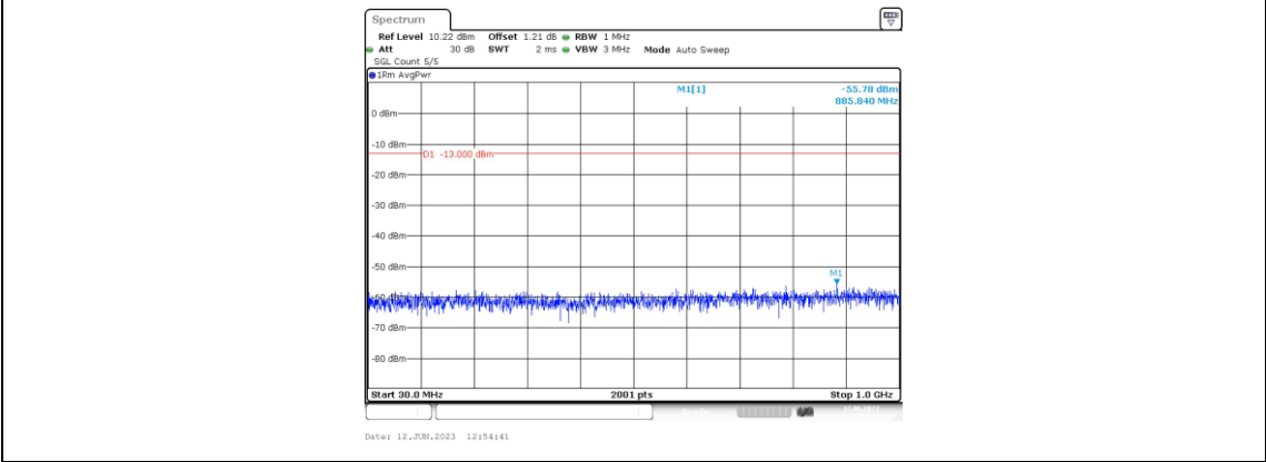
Band2-1.4MHz-QPSK-19193-1RB#0-Range3:30~1000MHz
