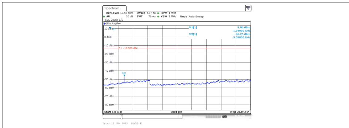
Band2-1.4MHz-QPSK-18607-1RB#0-Range4:1000~20000MHz
