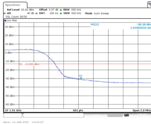
Band2-10MHz-QPSK-19150-50RB#0
