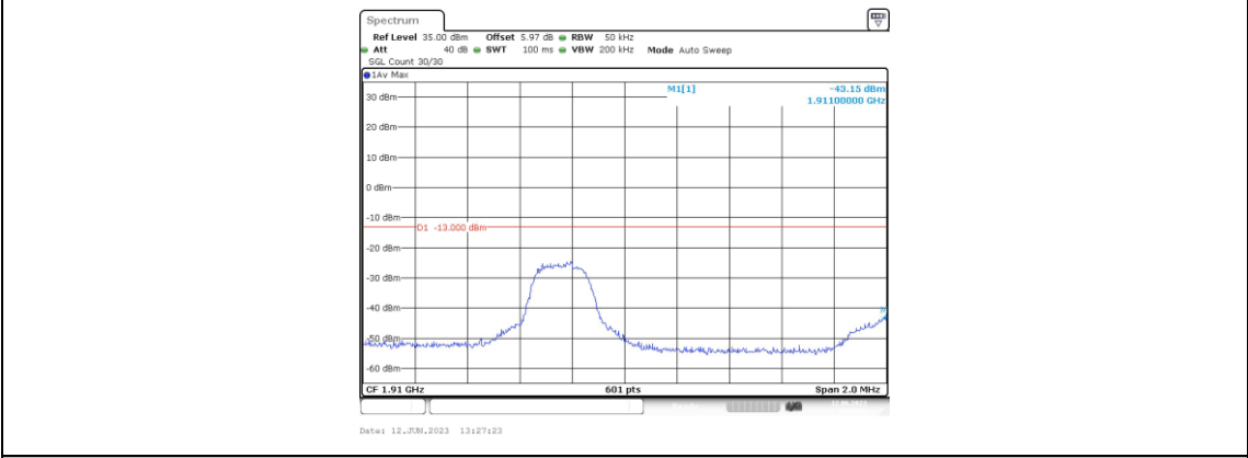
Band2-3MHz-16QAM-19185-1RB#0
