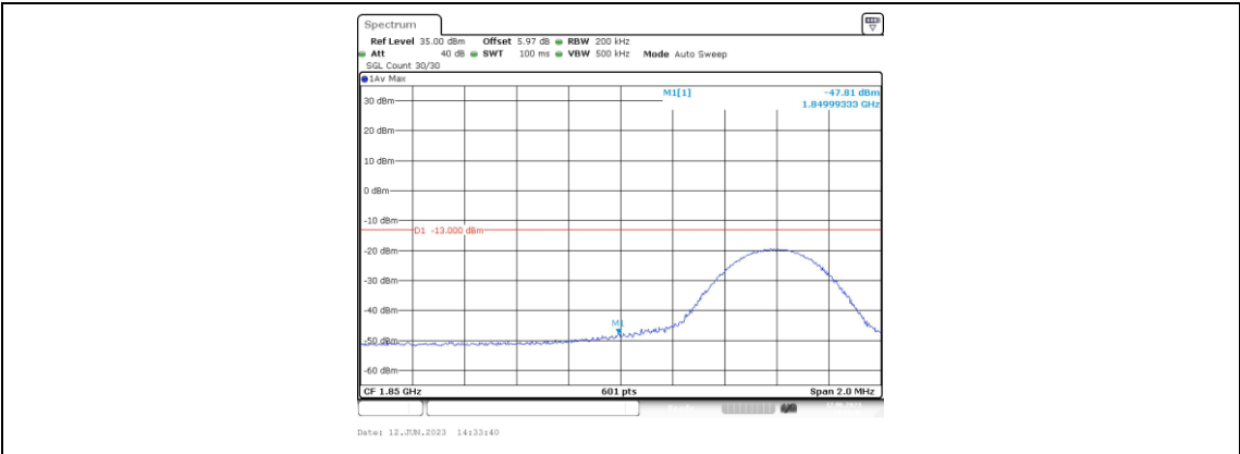
Band2-10MHz-QPSK-18650-1RB#49
