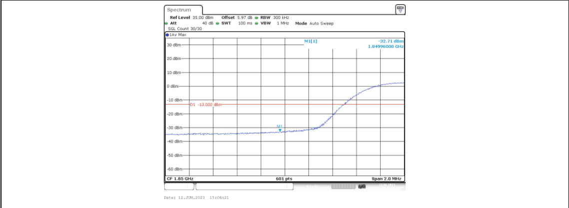
Band2-15MHz-16QAM-18675-75RB#0
