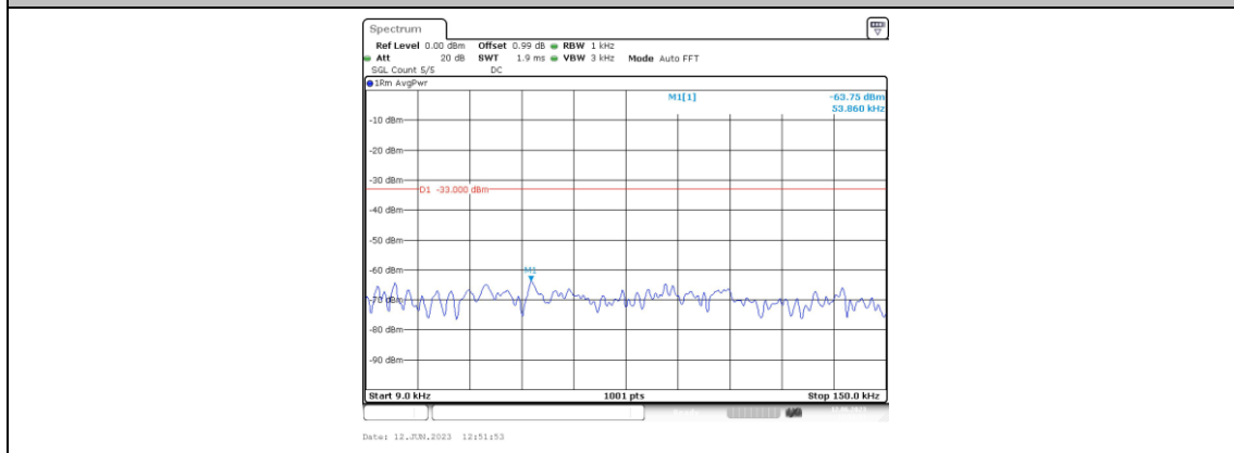
Band2-1.4MHz-16QAM-18607-1RB#0-Range1:0.009~0.15MHz
