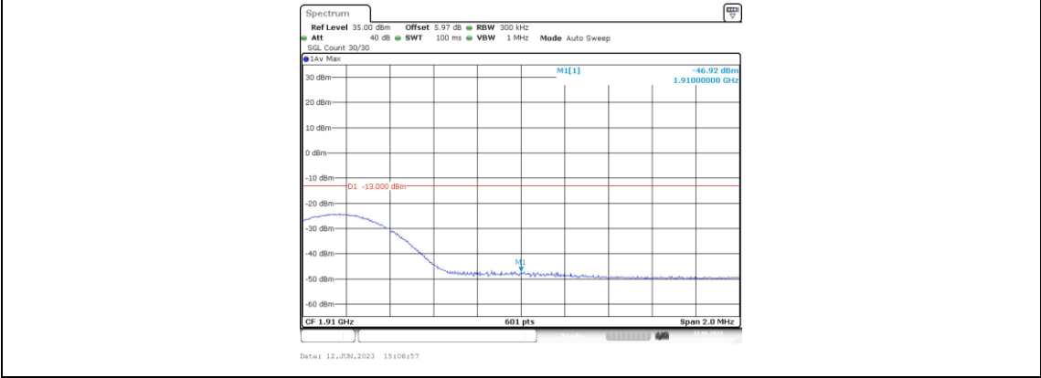
Band2-15MHz-QPSK-19125-1RB#0
