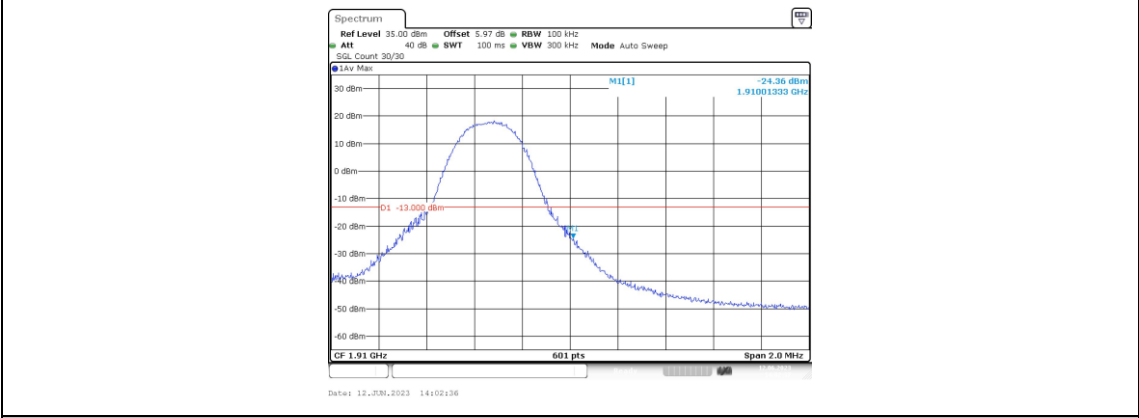
Band2-5MHz-16QAM-19175-1RB#24
