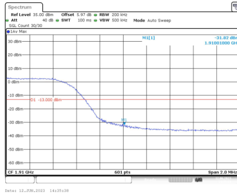
Band2-10MHz-16QAM-19150-50RB#0
