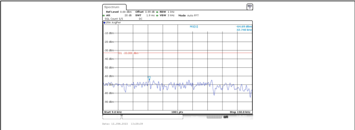
Band2-3MHz-QPSK-18615-1RB#0-Range1:0.009~0.15MHz
