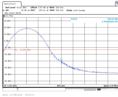
Band2-10MHz-16QAM-19150-1RB#49
