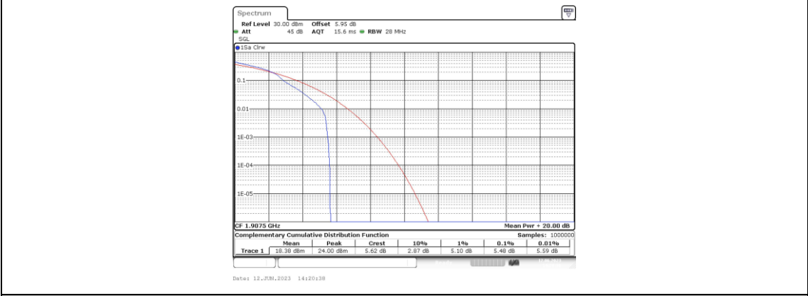
Band2-5MHz-16QAM-19175-25RB#0
