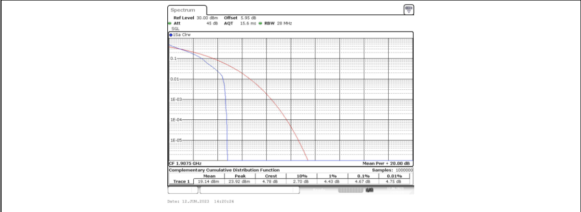
Band2-5MHz-16QAM-19075-25RB#0
