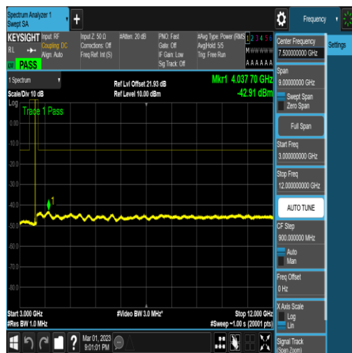
NTNV_N78-3450-3550_PC2_30_100_H_TID5_N/ A_3000_12000_#1
