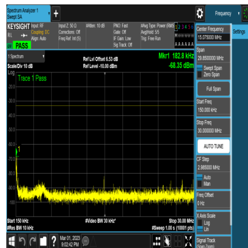
NTNV_N78-3450-3550_PC2_30_100_H_TID6_N/ A_0.15_30_#1
