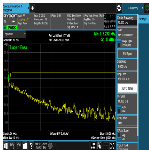
NTNV_N78-3450-3550_PC2_30_100_H_TID6_N/ A_0.009_0.15_#1
