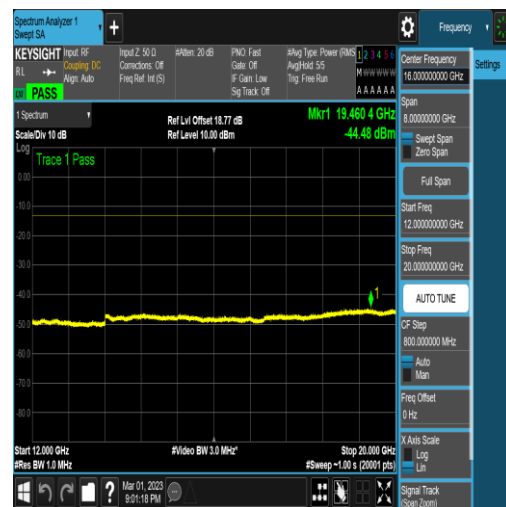
NTNV_N78-3450-3550_PC2_30_100_H_TID5_N/ A_12000_20000_#1
