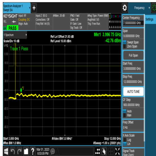
NTNV_N78-3450-3550_PC2_30_60_M_TID5_N/A _3000_12000_#1
