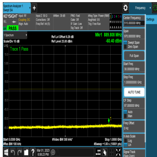
NTNV_N78-3450-3550_PC2_30_60_M_TID16_N/ A_30_1000_#1
