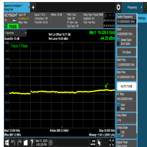
NTNV_N78-3450-3550_PC2_30_60_M_TID5_N/A _12000_20000_#1
