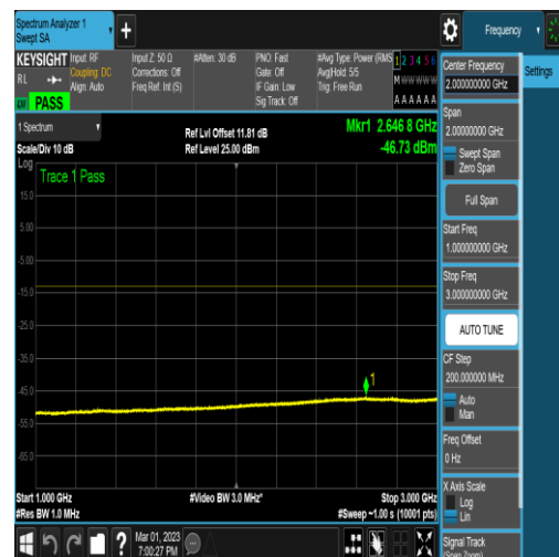
NTNV_N78-3450-3550_PC2_30_60_M_TID18_N/ A_1000_3000_#1
