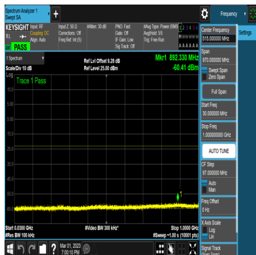
NTNV_N78-3450-3550_PC2_30_60_M_TID18_N/ A_30_1000_#1
