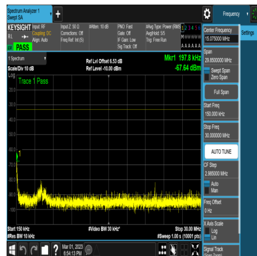
NTNV_N78-3450-3550_PC2_30_60_M_TID6_N/A _0.15_30_#1
