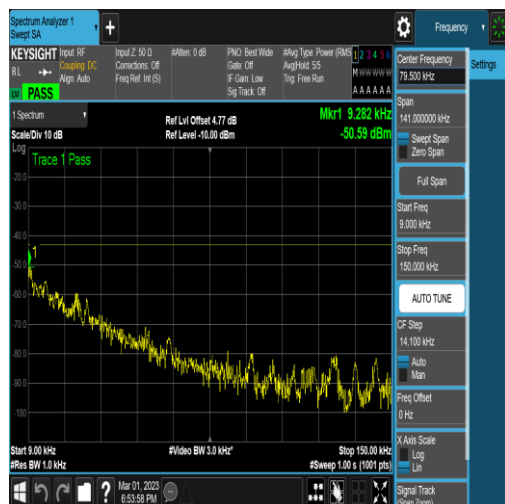
NTNV_N78-3450-3550_PC2_30_60_M_TID6_N/A _0.009_0.15_#1
