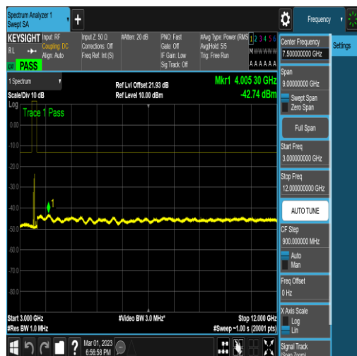
NTNV_N78-3450-3550_PC2_30_60_M_TID16_N/ A_3000_12000_#1
