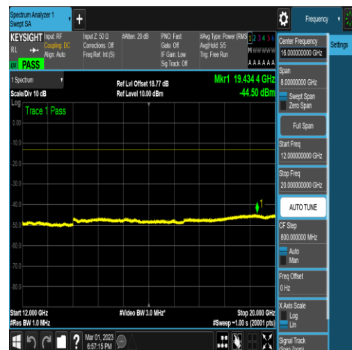
NTNV_N78-3450-3550_PC2_30_60_M_TID16_N/ A_12000_20000_#1
