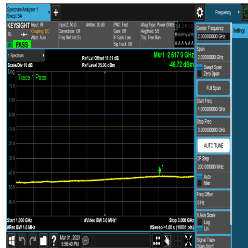
NTNV_N78-3450-3550_PC2_30_60_M_TID16_N/ A_1000_3000_#1
