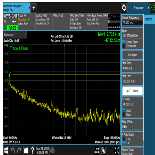
NTNV_N78-3450-3550_PC2_30_60_M_TID18_N/ A_0.009_0.15_#1
