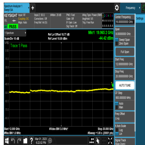
NTNV_N78-3450-3550_PC2_30_50_M_TID17_N/ A_12000_20000_#1
