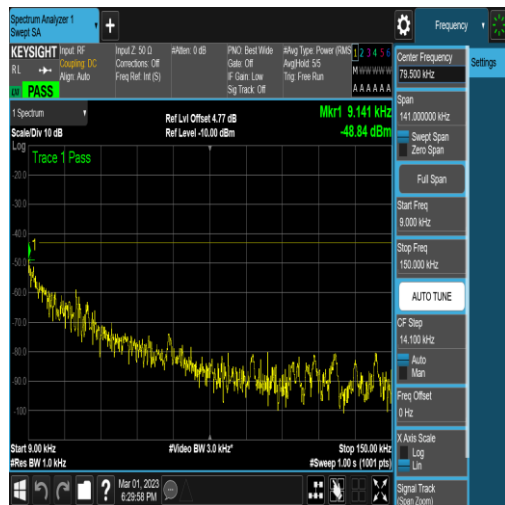
NTNV_N78-3450-3550_PC2_30_50_H_TID6_N/A _0.009_0.15_#1
