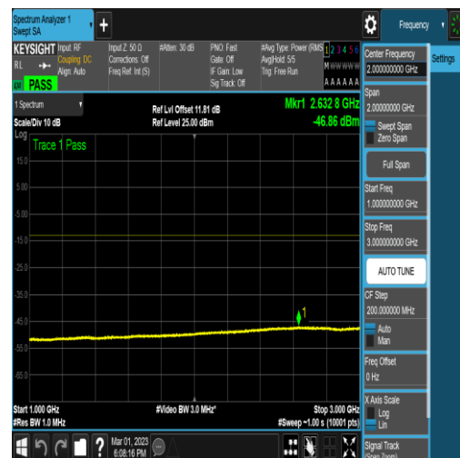
NTNV_N78-3450-3550_PC2_30_50_M_TID16_N/ A_1000_3000_#1
