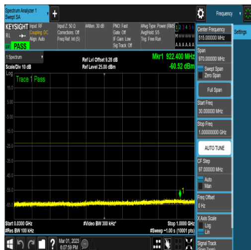
NTNV_N78-3450-3550_PC2_30_50_M_TID16_N/ A_30_1000_#1
