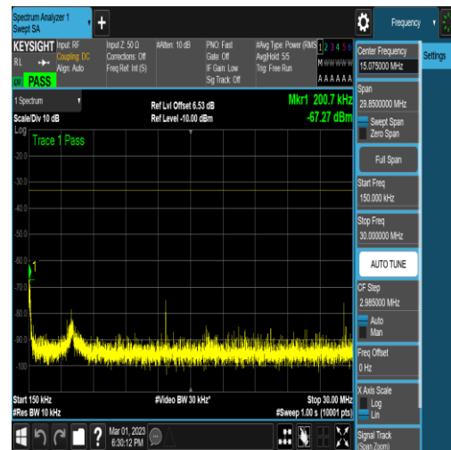
NTNV_N78-3450-3550_PC2_30_50_H_TID6_N/A _0.15_30_#1
