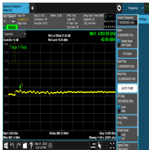
NTNV_N78-3450-3550_PC2_30_50_M_TID17_N/ A_3000_12000_#1
