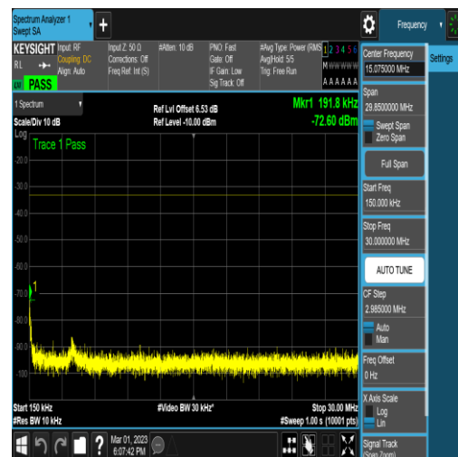
NTNV_N78-3450-3550_PC2_30_50_M_TID16_N/ A_0.15_30_#1
