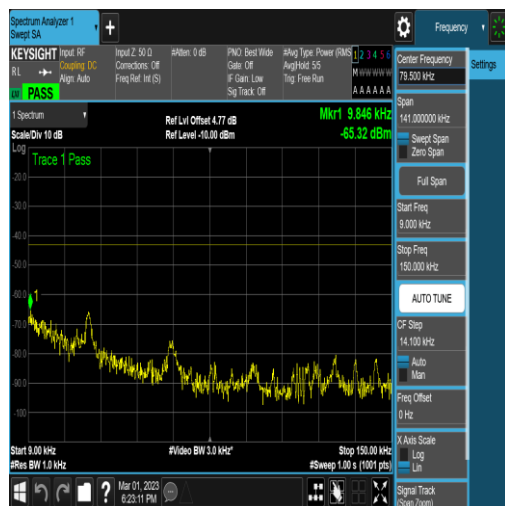
NTNV_N78-3450-3550_PC2_30_50_M_TID18_N/ A_0.009_0.15_#1
