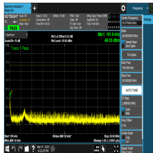
NTNV_N78-3450-3550_PC2_30_50_M_TID18_N/ A_0.15_30_#1
