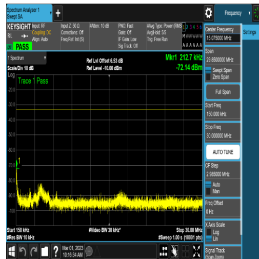
NTNV_N78-3450-3550_PC2_30_40_M_TID5_N/A _0.15_30_#1
