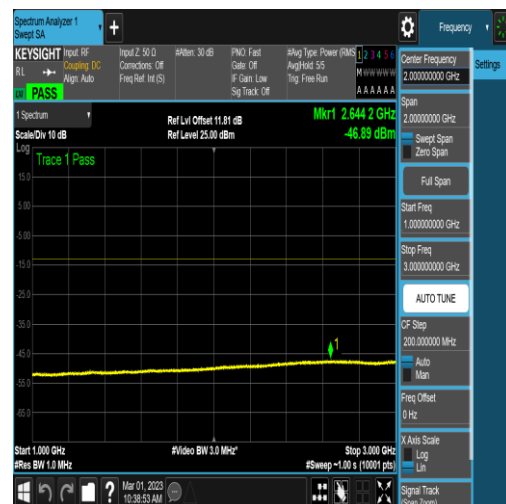
NTNV_N78-3450-3550_PC2_30_40_H_TID4_N/A _1000_3000_#1
