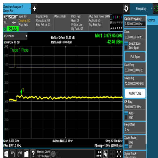
NTNV_N78-3450-3550_PC2_30_40_M_TID6_N/A _3000_12000_#1
