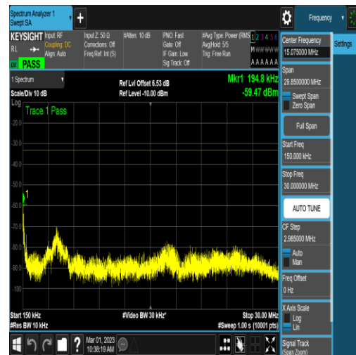
NTNV_N78-3450-3550_PC2_30_40_H_TID4_N/A _0.15_30_#1
