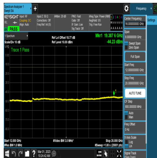
NTNV_N78-3450-3550_PC2_30_40_M_TID17_N/ A_12000_20000_#1
