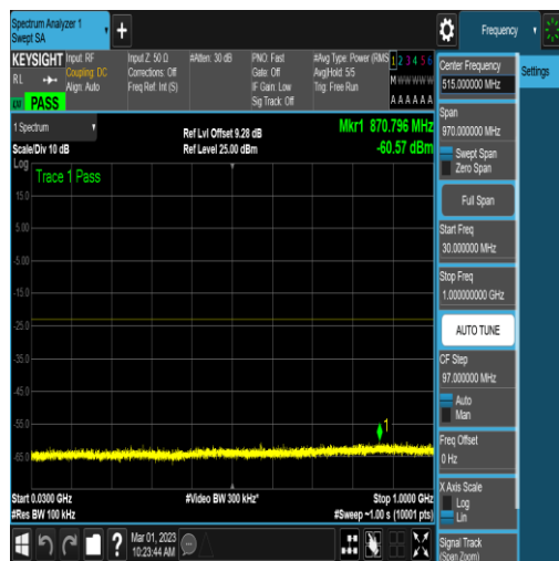
NTNV_N78-3450-3550_PC2_30_40_M_TID17_N/ A_30_1000_#1
