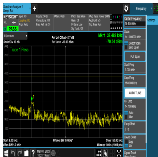
NTNV_N78-3450-3550_PC2_30_40_M_TID6_N/ A_0.009_0.15_#1
