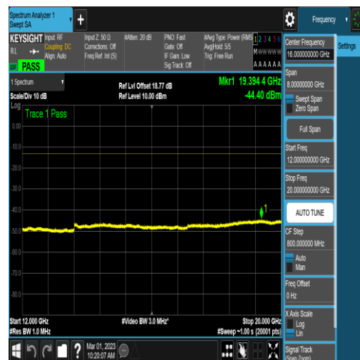
NTNV_N78-3450-3550_PC2_30_40_M_TID6_N/A _12000_20000_#1
