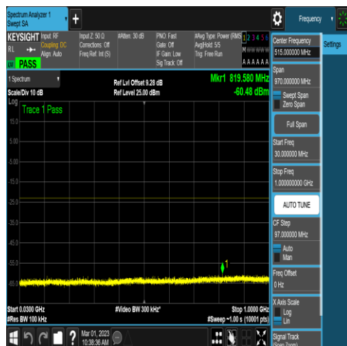
NTNV_N78-3450-3550_PC2_30_40_H_TID4_N/A _30_1000_#1
