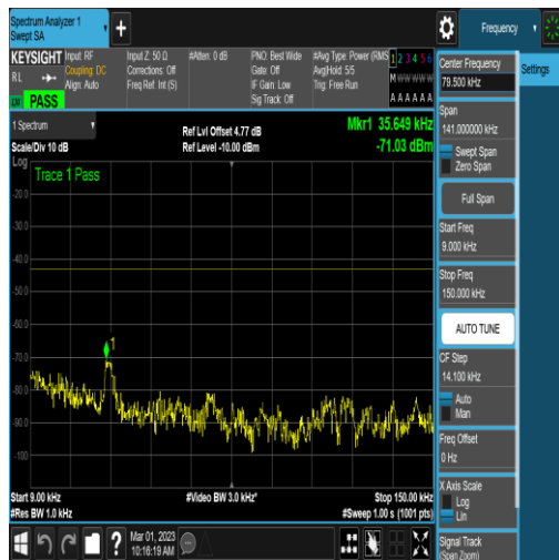
NTNV_N78-3450-3550_PC2_30_40_M_TID5_N/A _0.009_0.15_#1
