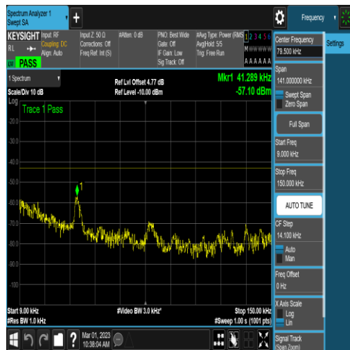
NTNV_N78-3450-3550_PC2_30_40_H_TID4_N/A _0.009_0.15_#1
