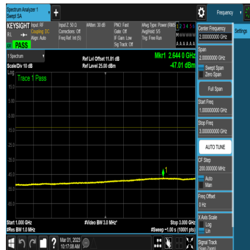
NTNV_N78-3450-3550_PC2_30_40_M_TID5_N/A _1000_3000_#1
