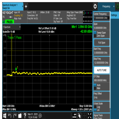
NTNV_N78-3450-3550_PC2_30_40_M_TID17_N/ A_3000_12000_#1
