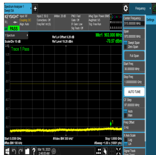
NTNV_DC_2A_n78A-3700-3800_PC3_30_5+90_ M+H_TID5_NS_01_30_1000_#1
