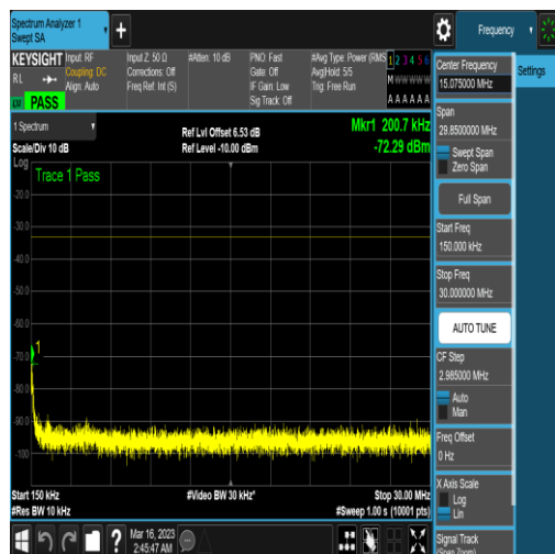
NTNV_DC_2A_n78A-3700-3800_PC3_30_5+90_ M+H_TID5_NS_01_0.15_30_#1
