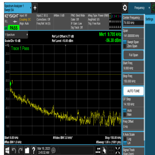
NTNV_DC_2A_n78A-3700-3800_PC3_30_5+90_ M+H_TID5_NS_01_0.009_0.15_#1
