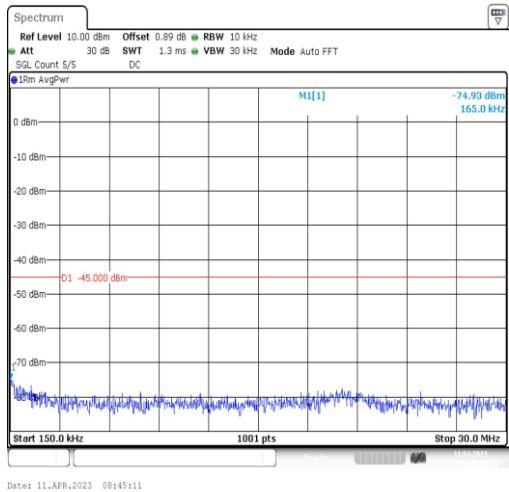
41-41-20MHz-20MHz-QPSK-QPSK-41292-41490-1RB#0-0RB#0-0.15~30MHz
