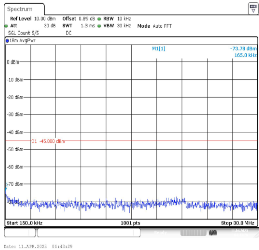
41-41-20MHz-5MHz-QPSK-QPSK-40595-40712-100RB#0-25RB#0-0.15~30MHz
