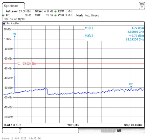
41-41-20MHz-5MHz-QPSK-QPSK-40595-40712-100RB#0-25RB#0-1000~20000MHz
