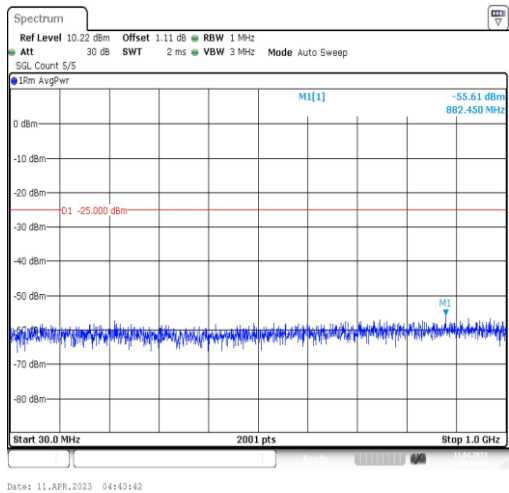
41-41-20MHz-5MHz-QPSK-QPSK-40595-40712-100RB#0-25RB#0-30~1000MHz
