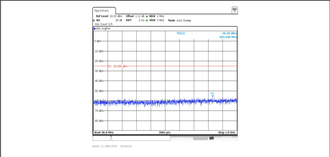
41-41-15MHz-20MHz-QPSK-QPSK-40523-40694-75RB#0-100RB#0-30~1000MHz
