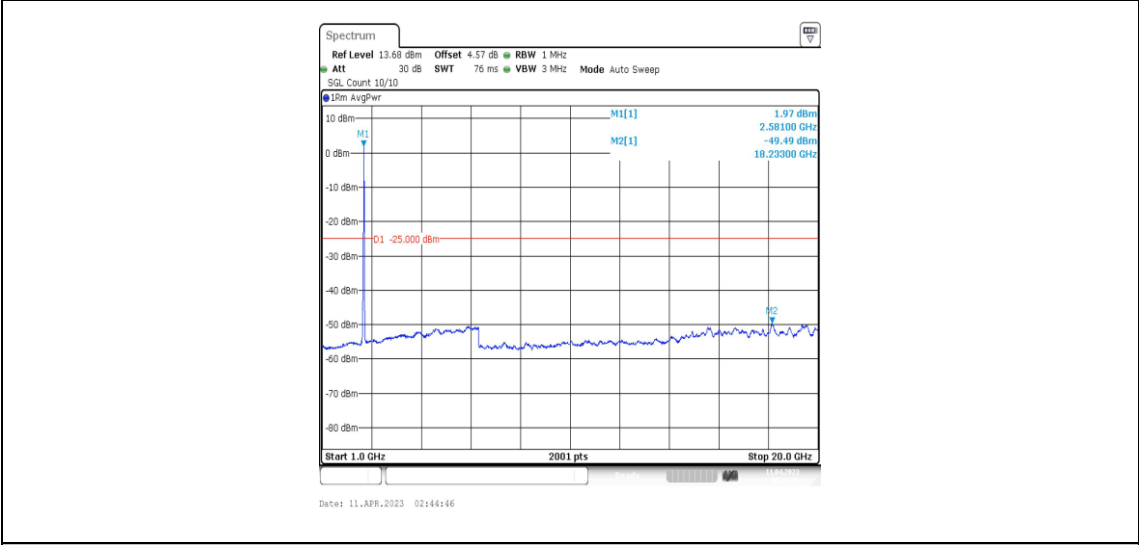
41-41-15MHz-20MHz-QPSK-QPSK-40523-40694-75RB#0-100RB#0-1000~20000MHz
