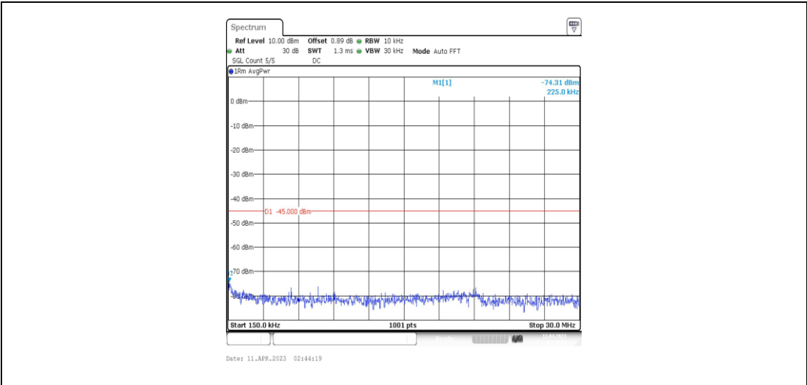
41-41-15MHz-20MHz-QPSK-QPSK-40523-40694-75RB#0-100RB#0-0.15~30MHz
