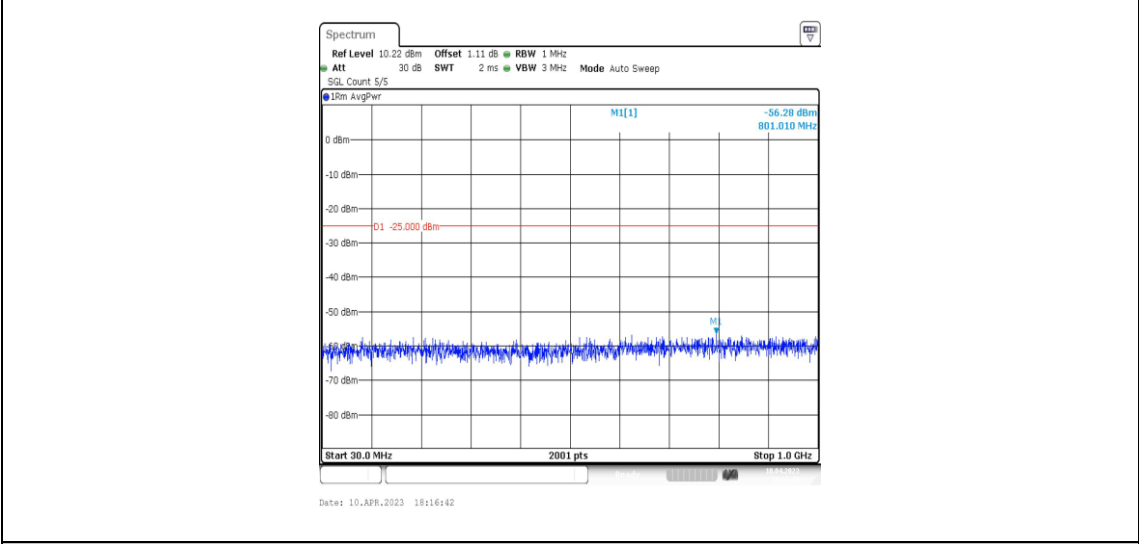
41-41-10MHz-15MHz-QPSK-QPSK-39703-39823-1RB#0-1RB#74-30~1000MHz
