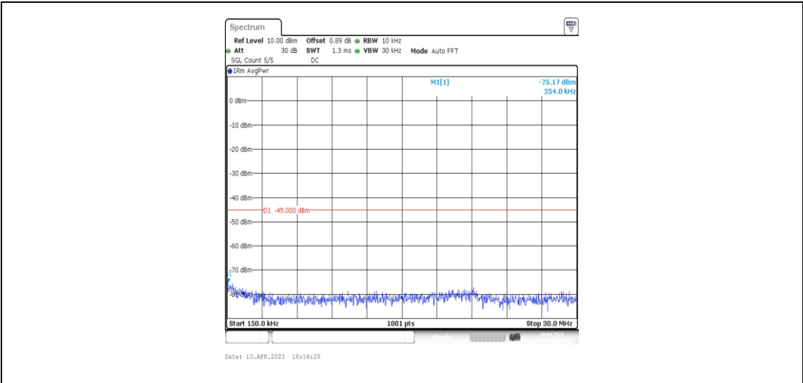
41-41-10MHz-15MHz-QPSK-QPSK-39703-39823-1RB#0-1RB#74-0.15~30MHz
