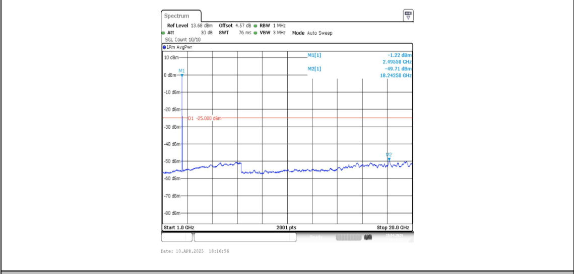
41-41-10MHz-15MHz-QPSK-QPSK-39703-39823-1RB#0-1RB#74-1000~20000MHz
