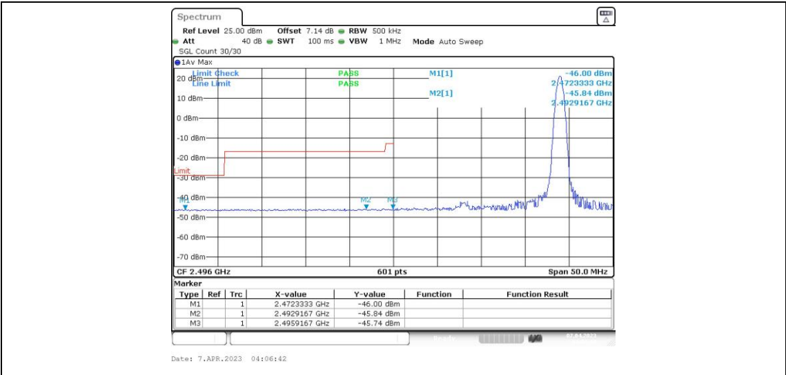
Band41-20MHz-QPSK-39750-100RB#0
