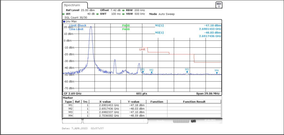
Band41-10MHz-QPSK-41540-1RB#49
