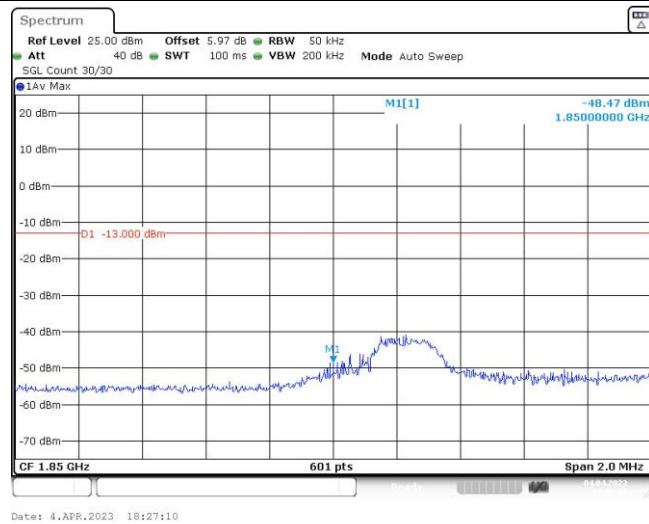
Band25-3MHz-16QAM-26055-15RB#0
