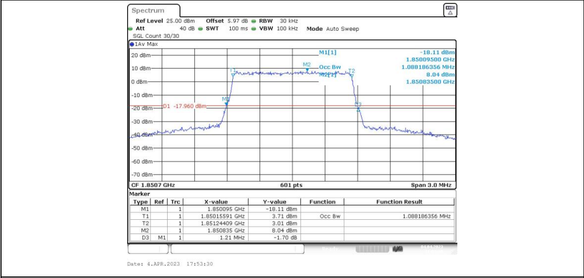
Band25-1.4MHz-16QAM-26365-6RB#0
