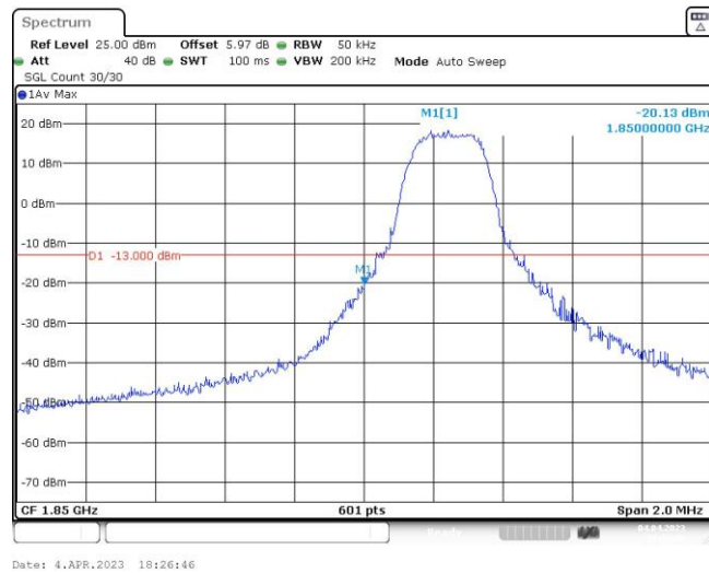
Band25-3MHz-16QAM-26055-1RB#14
