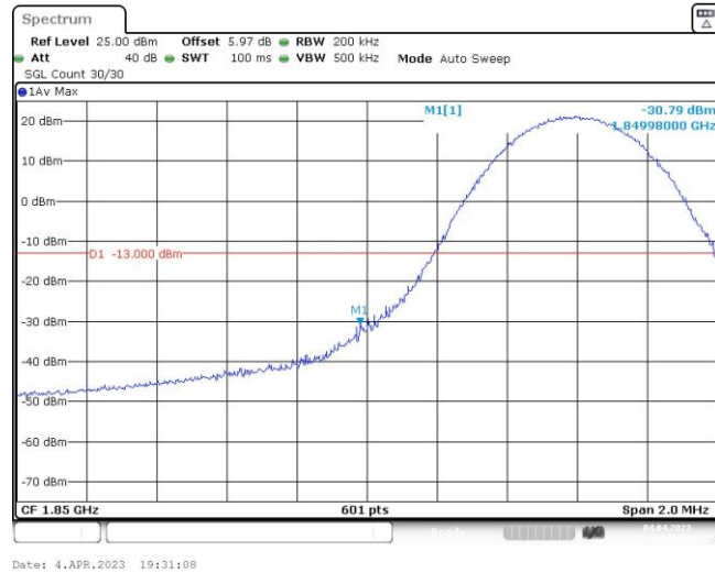
Band25-10MHz-16QAM-26090-1RB#49
