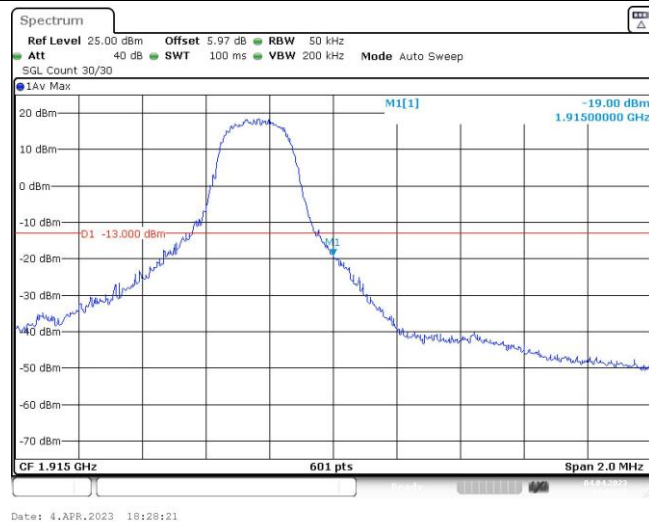
Band25-3MHz-QPSK-26675-15RB#0
