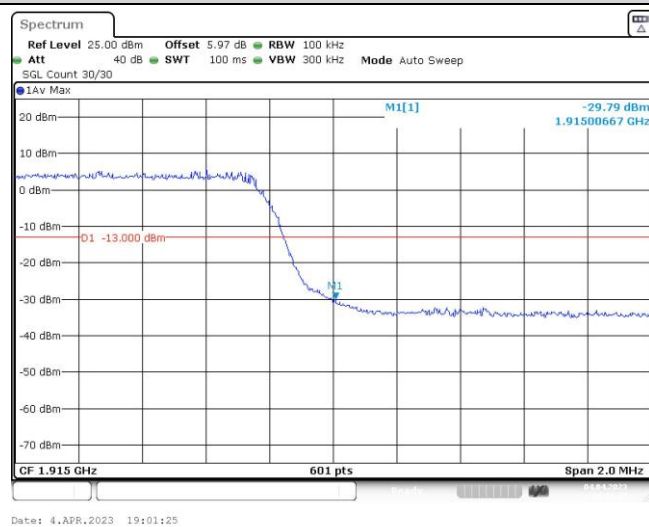
Band25-10MHz-QPSK-26090-1RB#0
