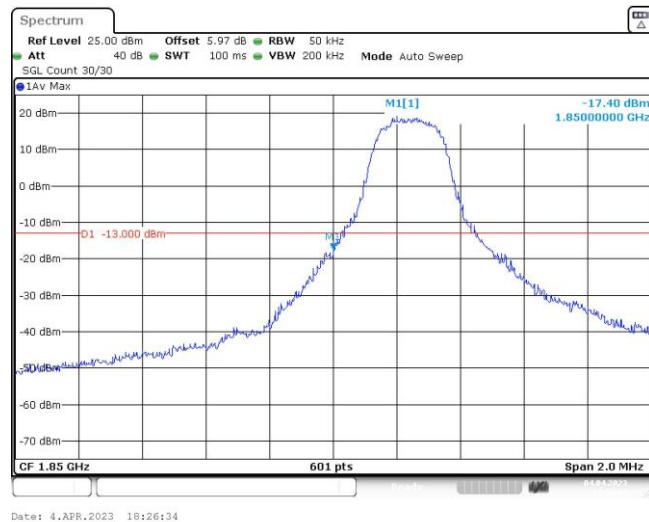
Band25-3MHz-QPSK-26055-1RB#14
