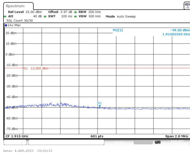
Band25-10MHz-16QAM-26640-1RB#49
