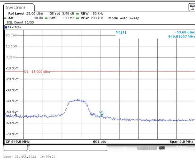
Band5-3MHz-16QAM-20635-1RB#14
