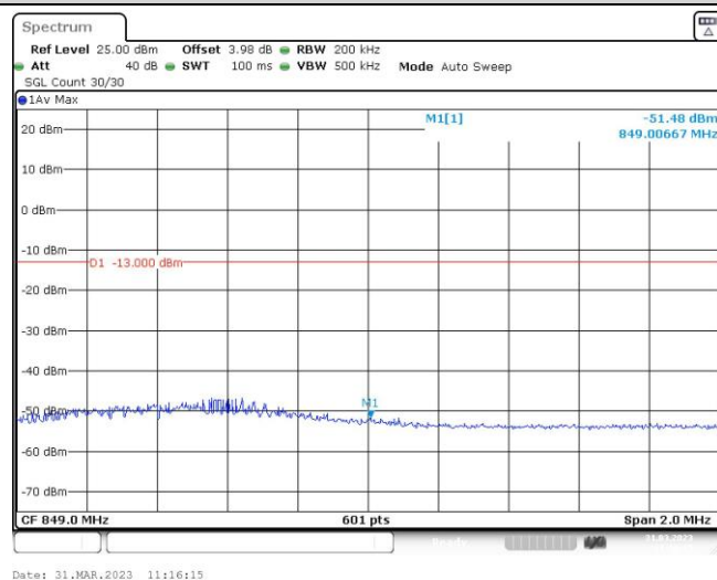
Band5-10MHz-16QAM-20600-1RB#49
