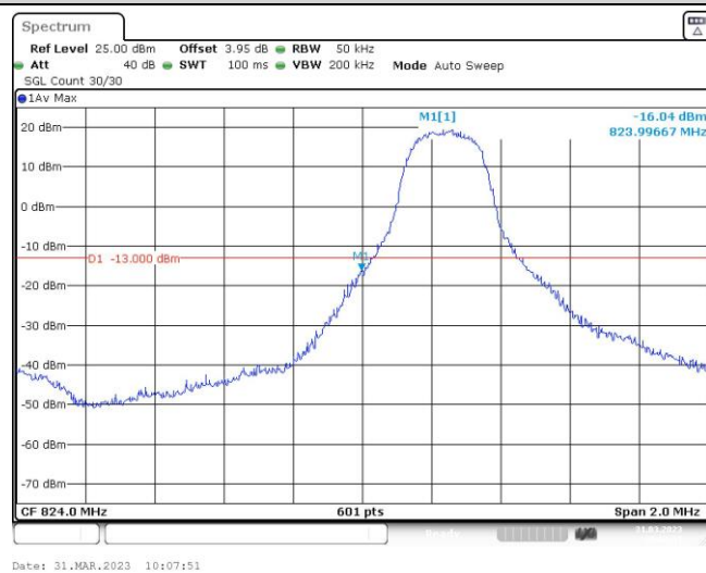
Band5-3MHz-QPSK-20415-1RB#14
