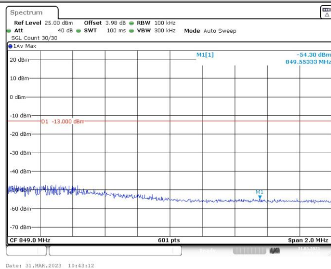
Band5-5MHz-16QAM-20625-1RB#24
