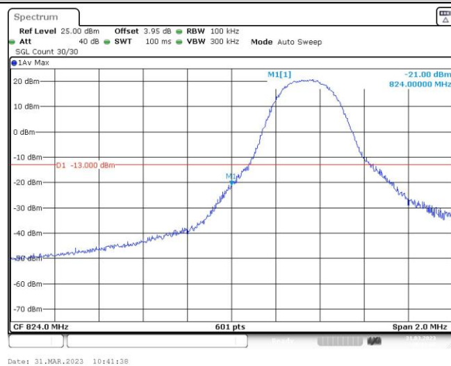
Band5-5MHz-QPSK-20425-1RB#24
