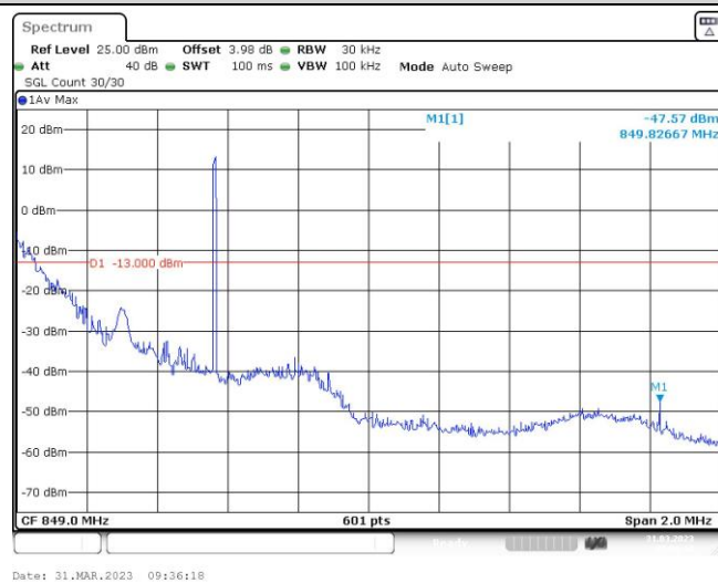
Band5-1.4MHz-QPSK-20643-1RB#5
