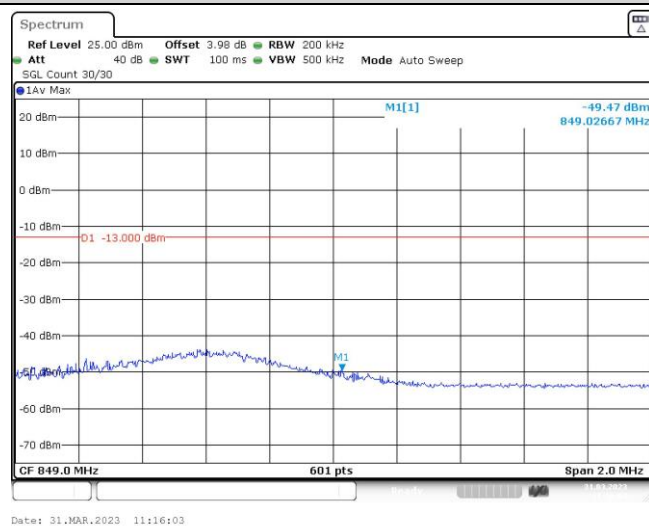
Band5-10MHz-QPSK-20600-1RB#49
