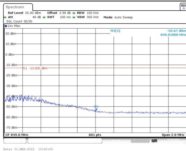
Band5-5MHz-QPSK-20625-1RB#24
