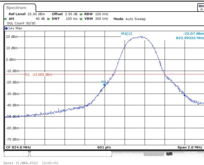
Band5-5MHz-16QAM-20425-1RB#24
