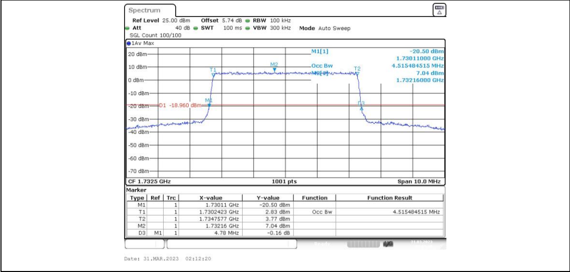
Band4-5MHz-16QAM-20375-25RB#0
