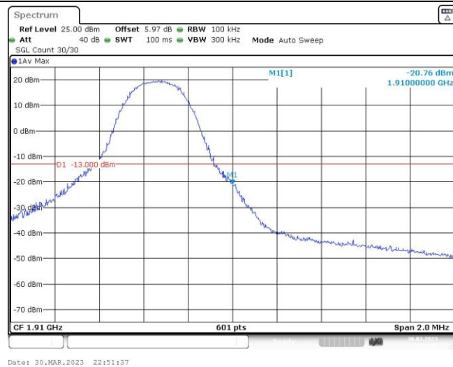
Band2-5MHz-QPSK-19175-25RB#0
