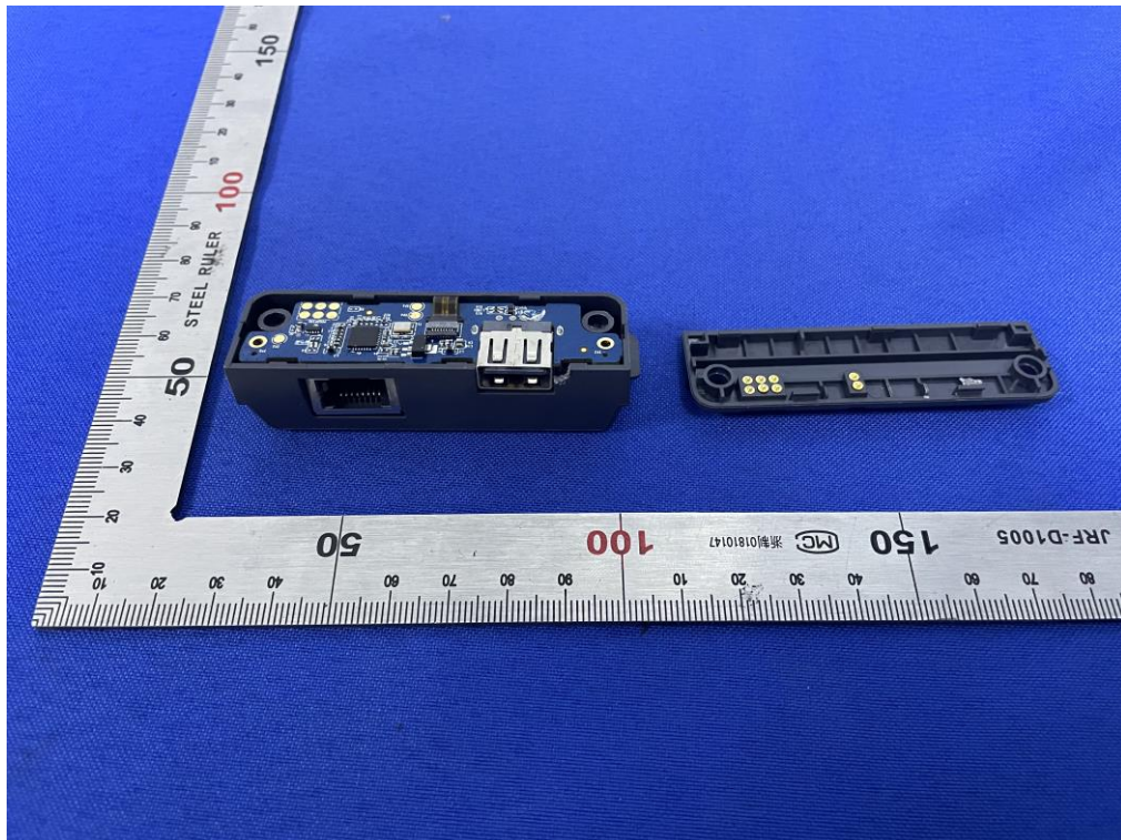
RJ45+USB(Open)
