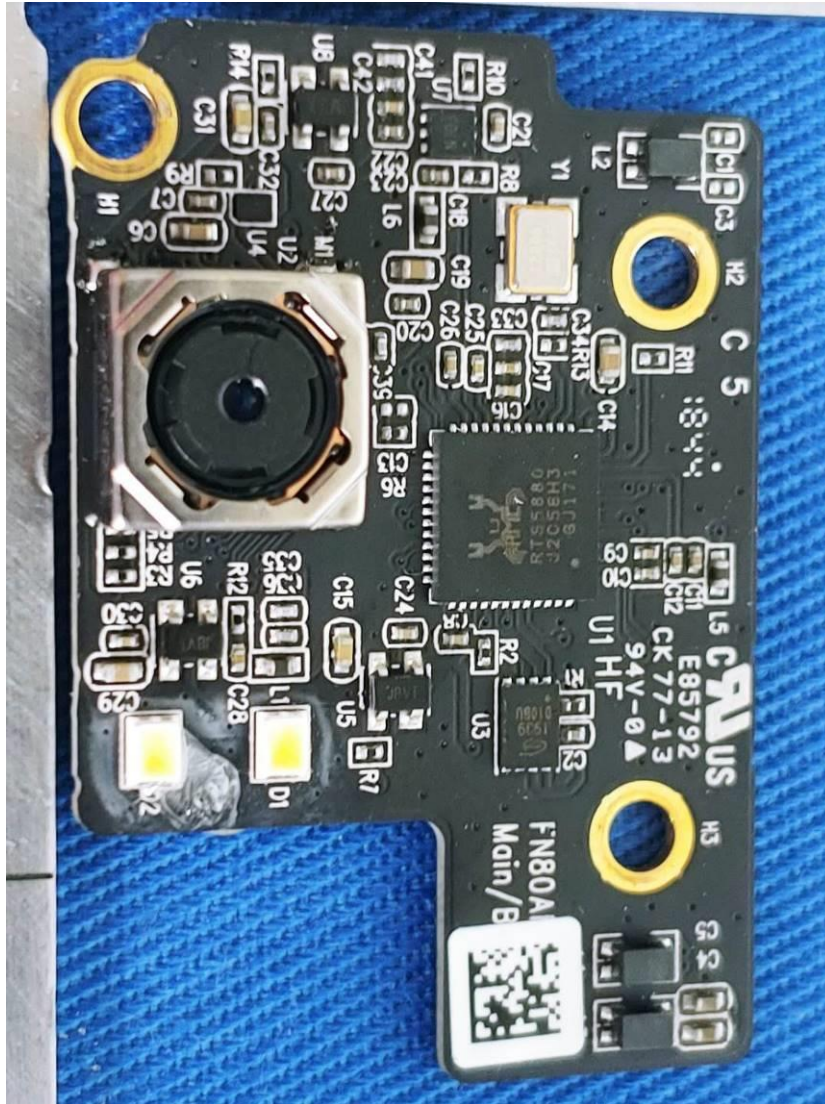
Camera
