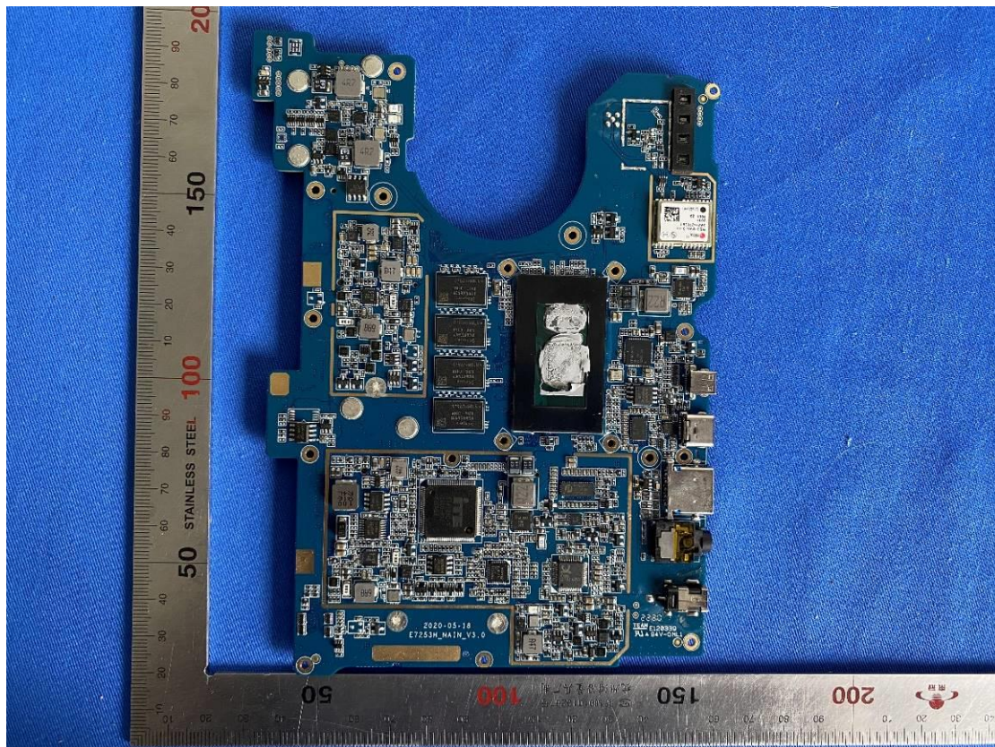
Main chip
