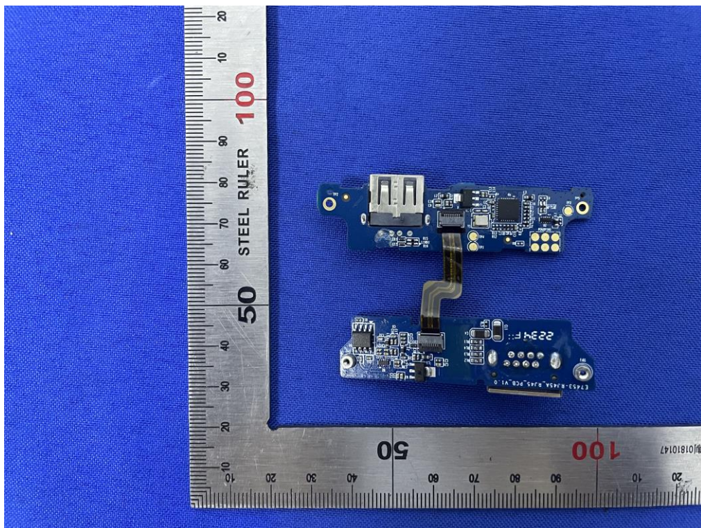
RJ45+USB (Internal Photo-2)
