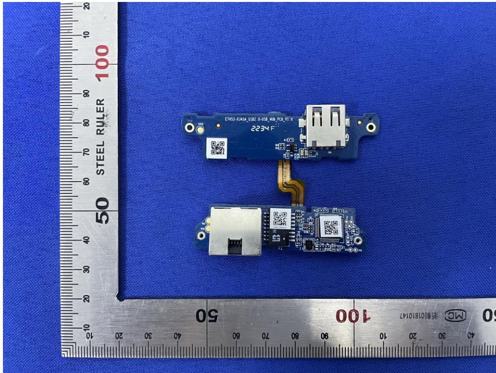
RJ45+USB (Internal Photo-1)
