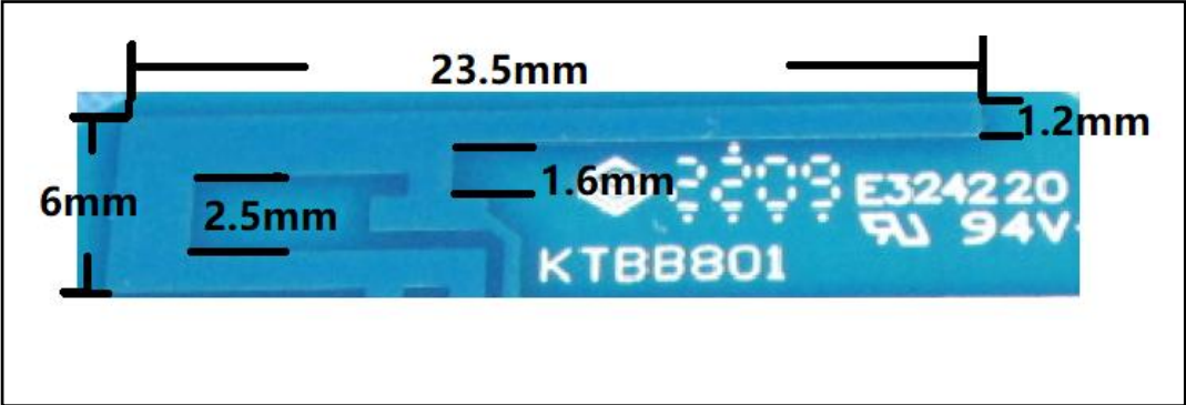
产品规格图(Antenna Specification chart)
