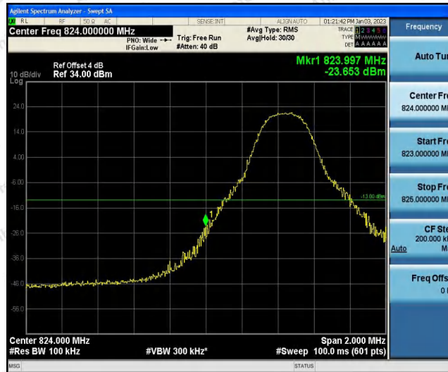
Band5-5MHz-QPSK-20425-1RB#24
