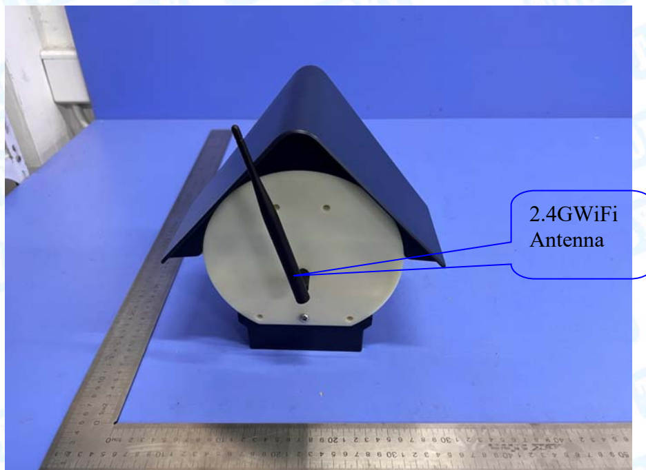
Photo 4 Appearance of EUT
