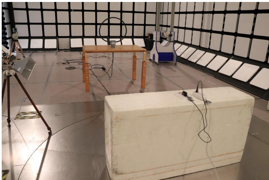
Photograph 5. Radiated Emissions 9 kHz – 30 MHz
