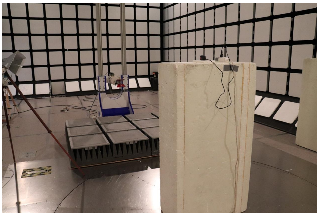
Photograph 8. Radiated Emissions 1 – 18 GHz
