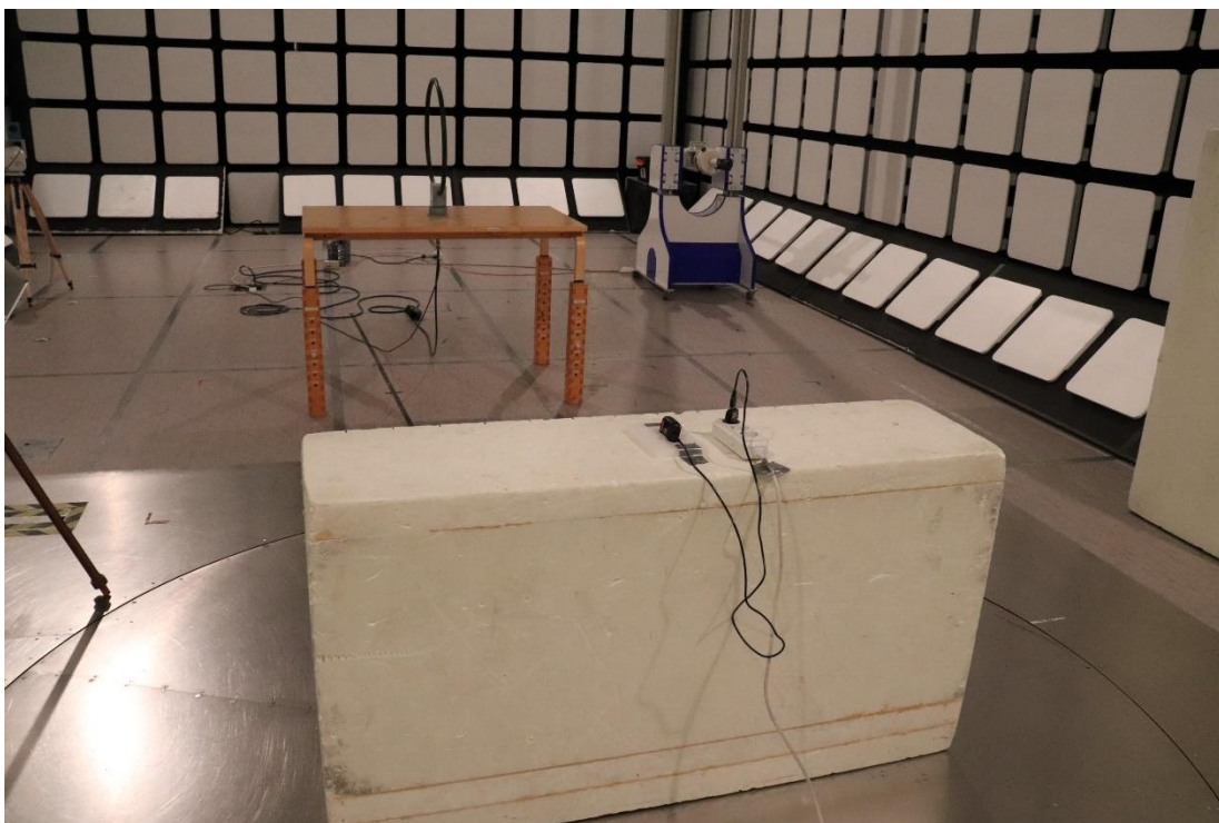
Photograph 6. Radiated Emissions 9 kHz – 30 MHz
