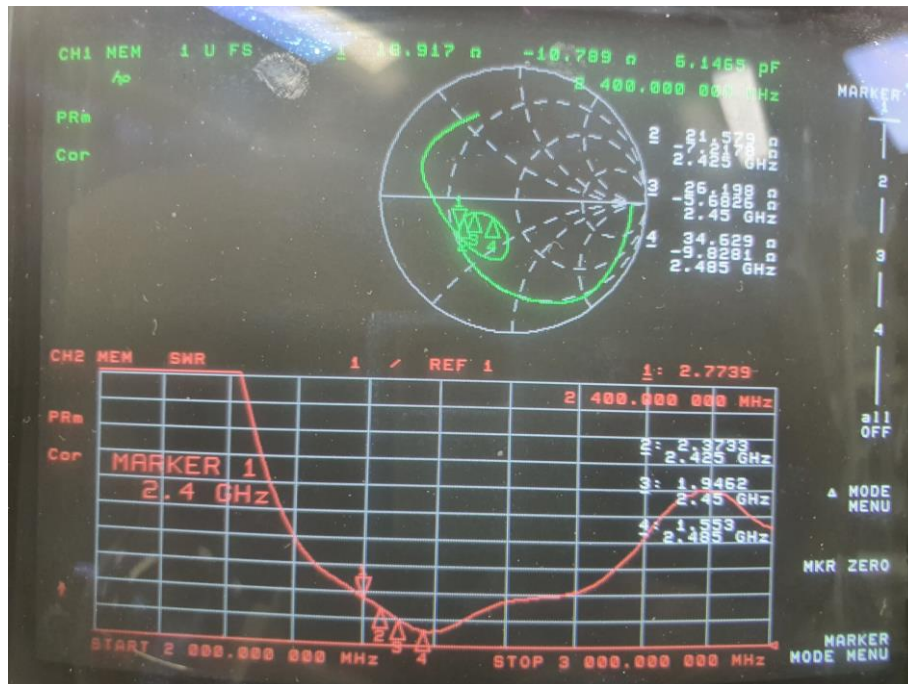
Smith chart & VSWR
