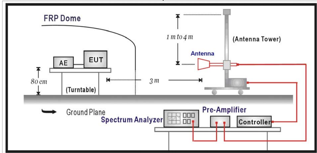
RadiatedSpuriousMeasurement:
