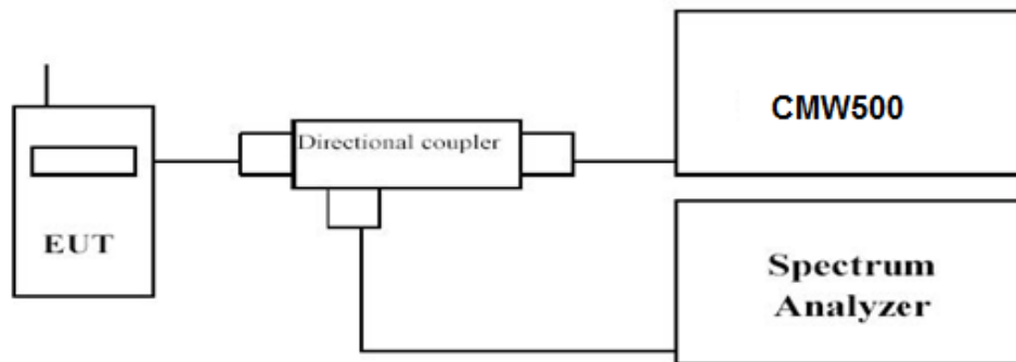
ConductedSpuriousMeasurement:
