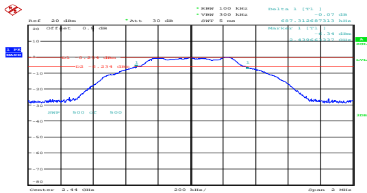
Middle 0.687MHz
