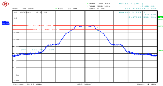
High 0.683MHz
