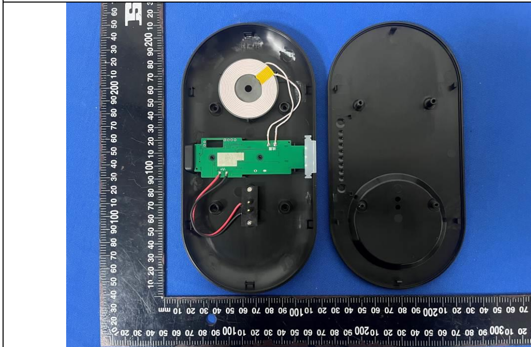
Internal photos
