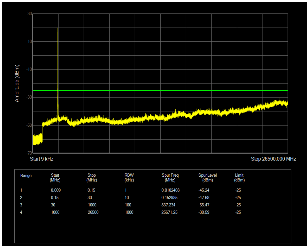
Band41(2555-2655) QPSK BW=15MHz Channel=41165 RB Size=1 Position=#0
