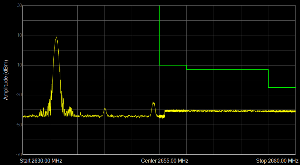
Band41(2555-2655) QPSK BW=20MHz Channel=41140 RB Size=1 Position=#0
