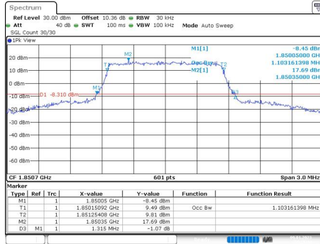
Band25-1.4MHz-QPSK-26047-6RB#0
