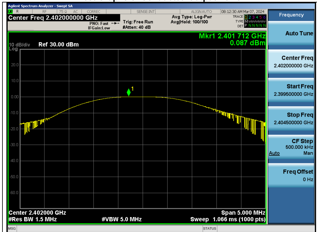
Test_Graph_ANT1_2402_Peak Power
