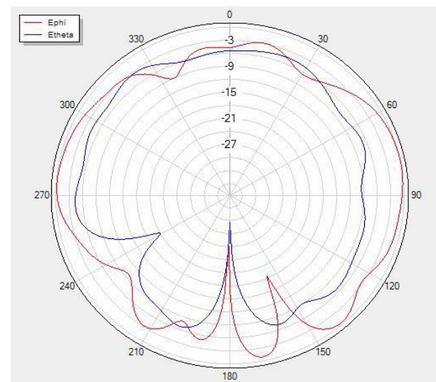
Phi=0 freq=2440MHz
