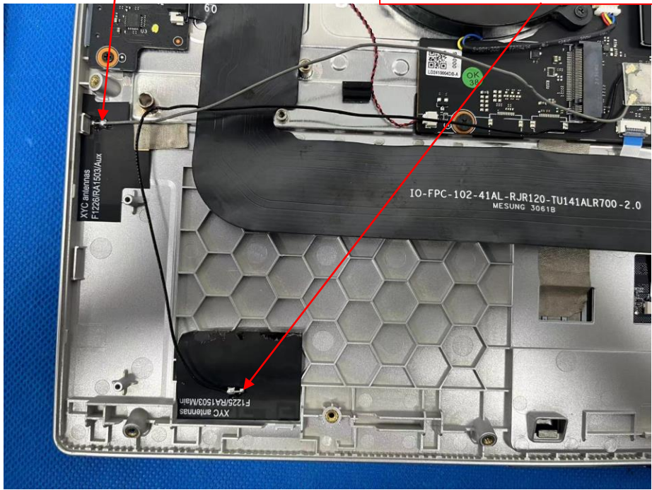
ANT A: BT/BLE/2.4G WIFI/5G WIFI
