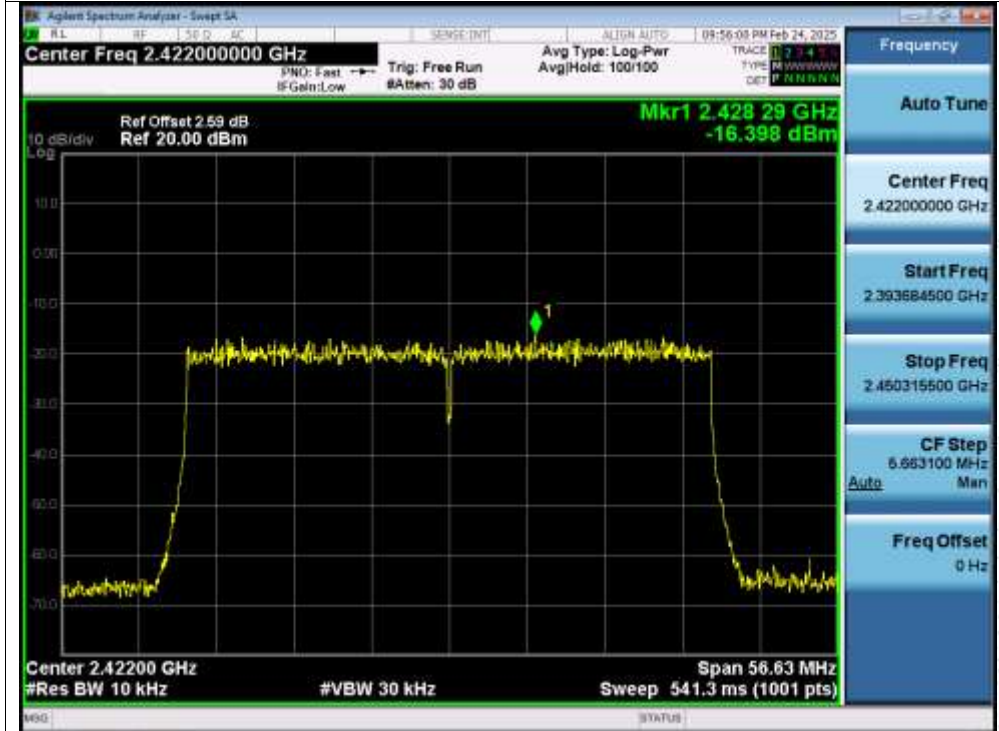
PSD NVNT ax40 2422MHz
