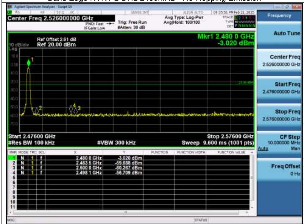
Band Edge NVNT 2-DH1 2480MHz No-Hopping Emission
