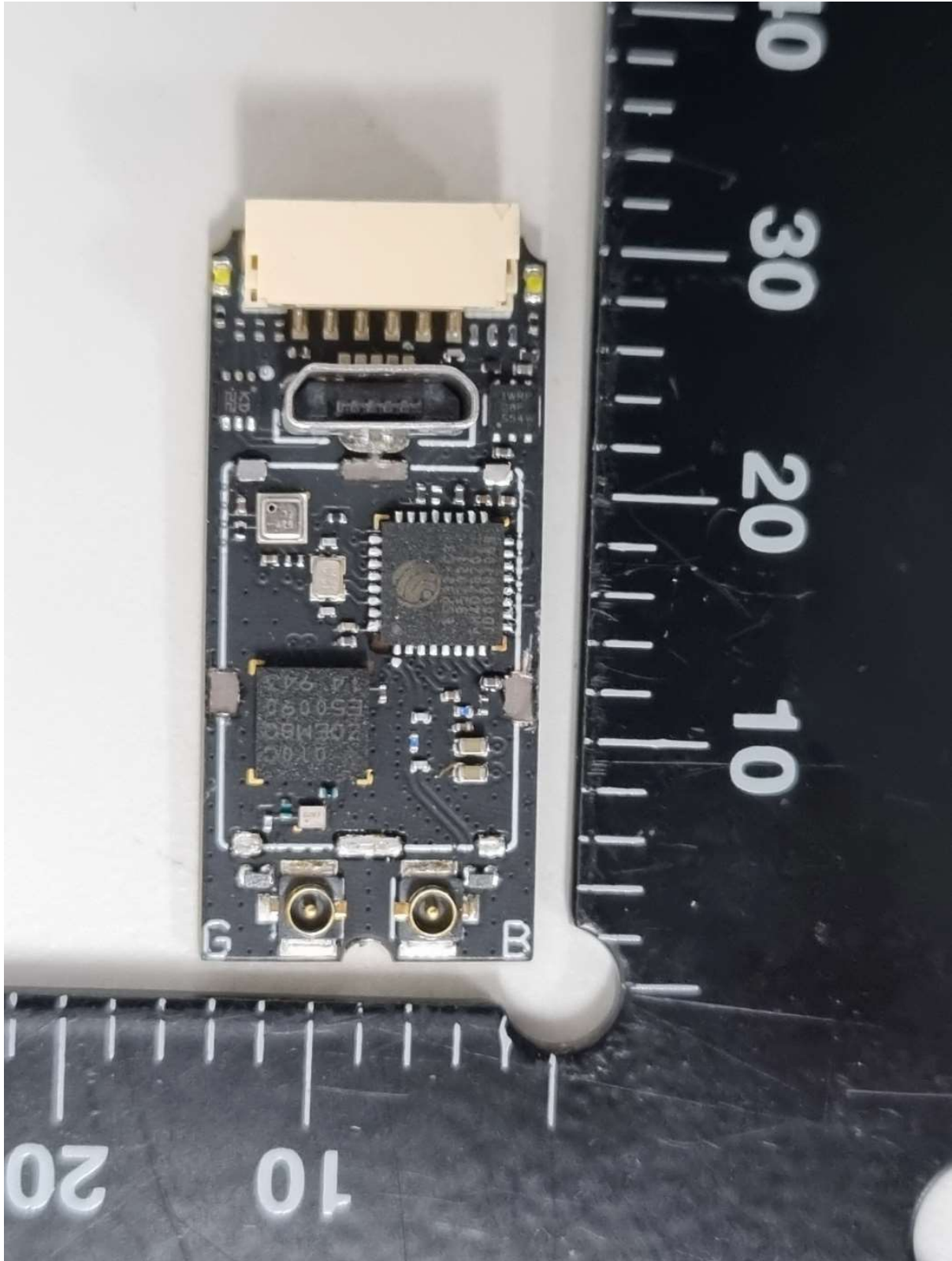
Main Board(Front)
