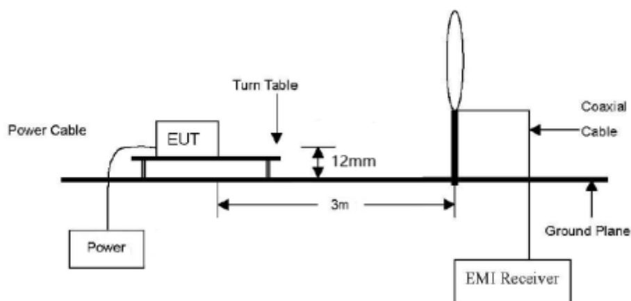
Test set-up of radiated disturbance (Below 30MHz)
