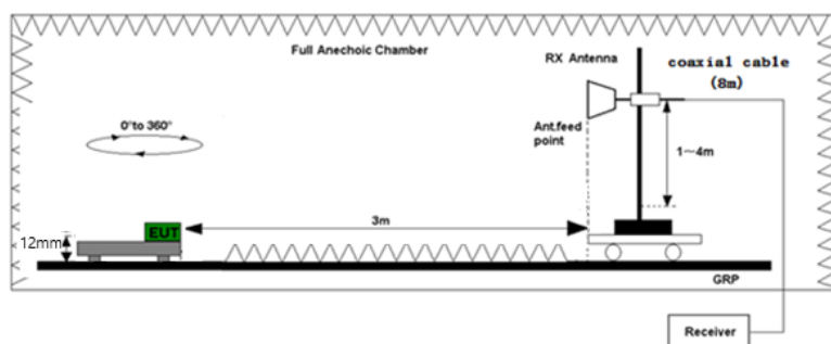
Test set-up of radiated disturbance (Above 1GHz)
